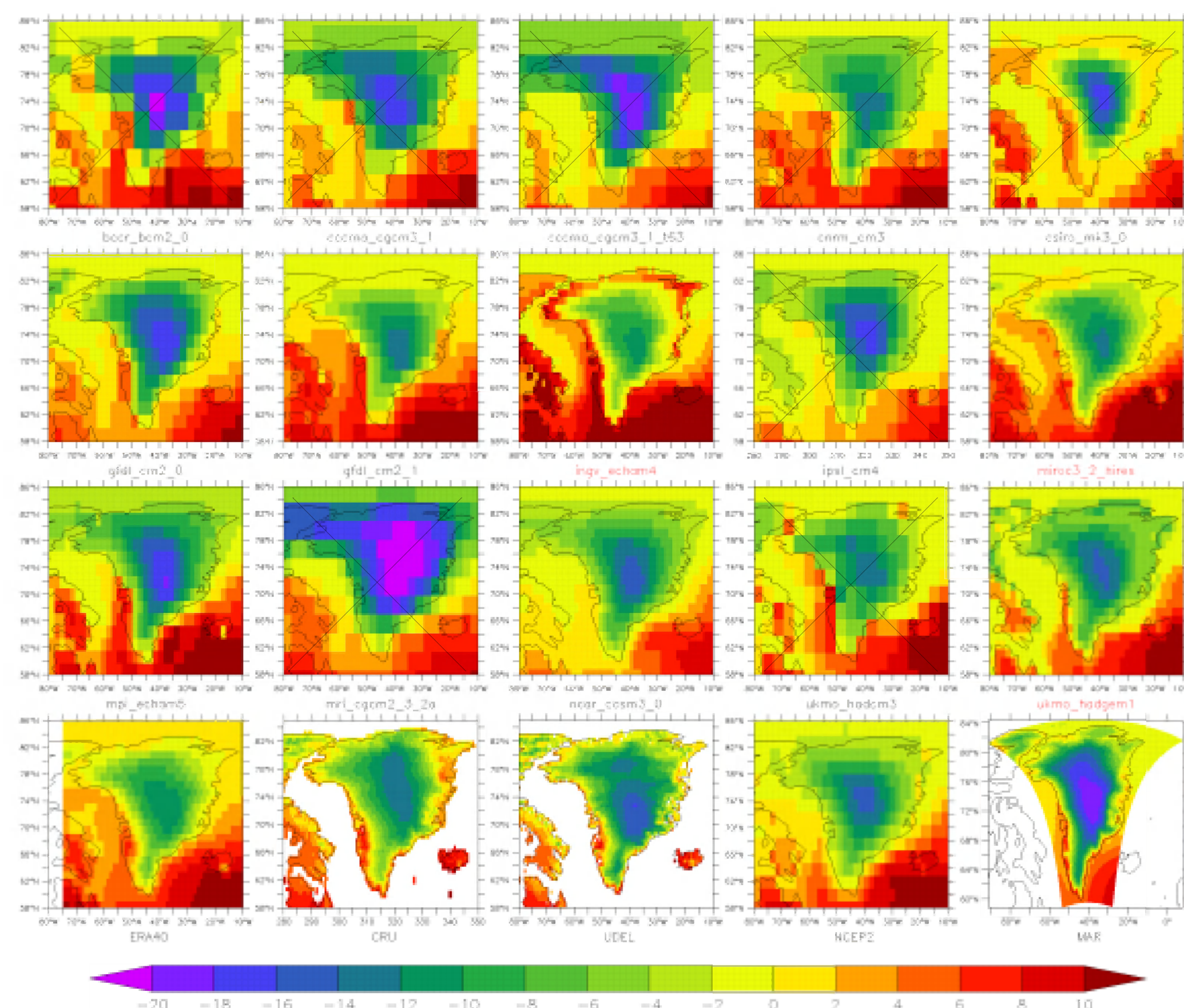
Fig 2 : Summer temperature (°C) for the 1970-1999 period simulated by some IPCC AR4 AOGCM's, by reanalyses (ERA-40, NCEP2) and from climatological time series (CRU, UDEL) and simulated by the MAR model.
