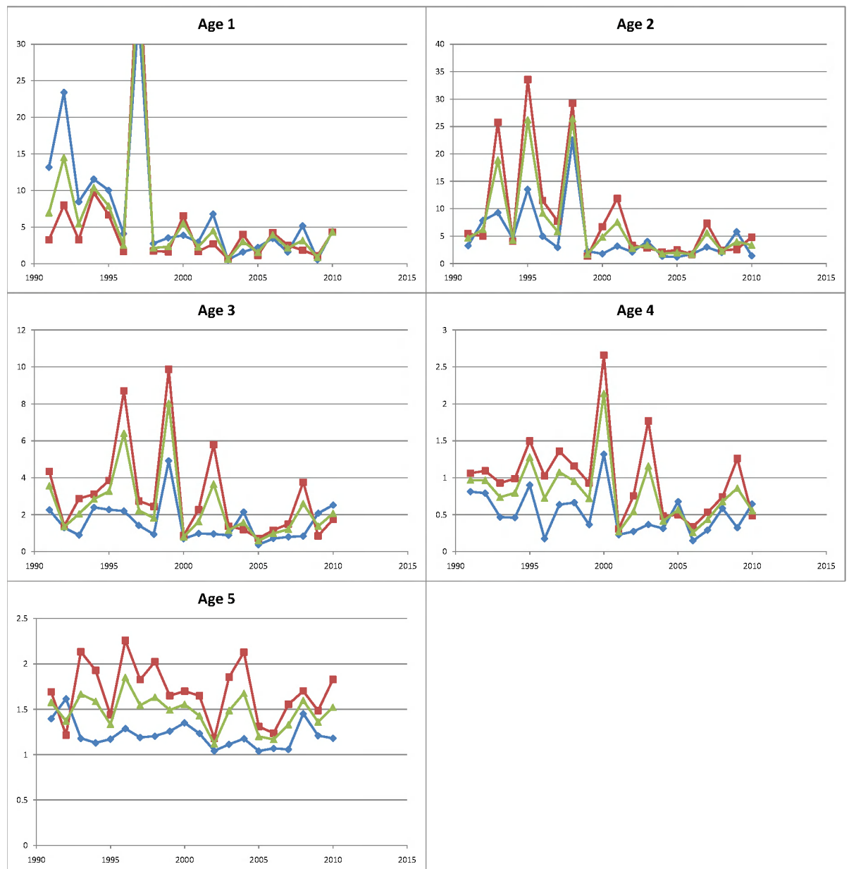
Figure 3.2.5. Cod in Subarea IV and Divisions IIIa (Skagerrak) and VIId. The time-series of IBTSq1 average survey catch rates at age for the northern ( \geq 56^\circ , red) and southern (blue) North Sea and the average index (green).
