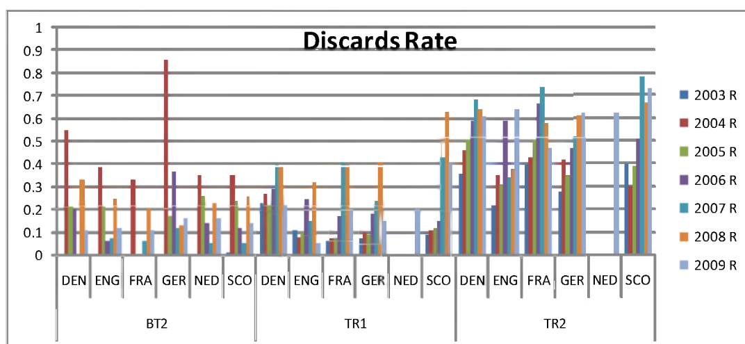
Figure 3.3.4. Cod discards rate in weight in area IV, IIIa and VIId broken down by main EU Member state and gear. Source STECF SG-MOS 10-05.
