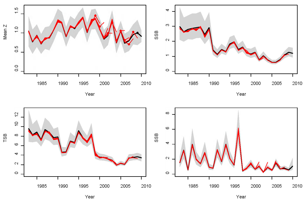
Figure 4.1.3. Retrospective SURBA model fits for North Sea cod: stock summary. In each plot, the black line gives the full time-series estimate (with 90% confidence interval as a grey band). Retrospective estimates are given as red lines. For mean Z (top left), the final-year estimate for each run is based on a three-year mean (rather than directly on data), so the penultimate-year estimates are highlighted with points as these represent the appropriate retrospective comparison. SSB, TSB and recruitment are all presented on a relative scale.
