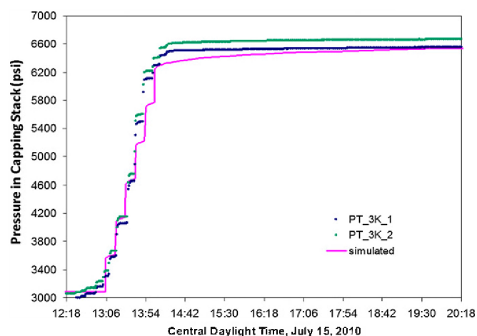
Fig. 2. Wellhead pressure measured during and immediately after closure of the capping stack on the Macondo Well on July 15, 2010 as measured by pressure gauges installed on the capping stack (PT_3K_1 and PT_3K_2). The pink line denotes pressure simulated by the initial (square) reservoir model assuming a well with no leaks. (Modified from ref. 18 with permission of the National Ground Water Association, Copyright 2011.)
