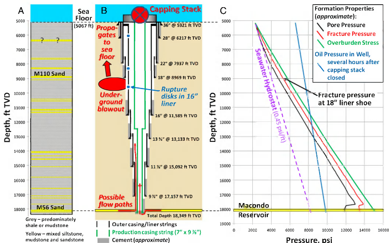
Fig. 1. (A) Schematic lithologic section for the Macondo Well based upon analysis of data acquired during drilling (Source: BP). Depths are total vertical depth (TVD) below the Deepwater Horizon rig floor [75 ft (23 m) above mean sea level]. (B) Completion diagram for the Macondo Well showing outer nested casing and liner strings cemented in place during drilling and production casing cemented across the Macondo Reservoir (M56 sand, yellow). Possible oil flow paths during the blowout are shown in red, which were either inside the production casing, between the production casing and the outer casing/liner strings, or both. (Based on data from ref. 30.) (C) Approximate in situ pore pressure, fracture pressure, and overburden stress profile for the Macondo Well showing that pore fluid pressures at the Macondo site are overpressured relative to a seawater hydrostat. The blue line shows the approximate oil pressure in the wellbore corresponding to a capping stack pressure of 6,600 psi, which was observed several hours after the well was shut in (calculated for an oil pressure gradient in the well of 0.25 psi/ft). (Modified from ref. 31. Overburden stress and oil pressure gradient from BP.).
