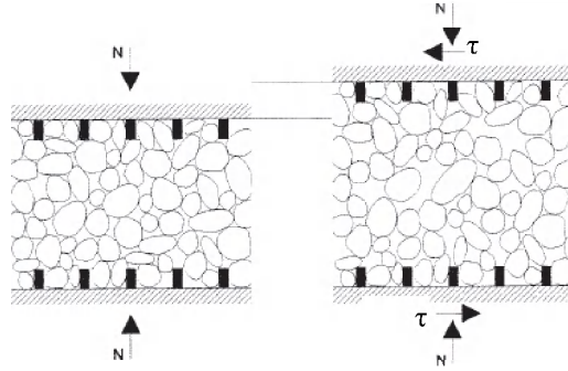
Figure 4. Increase of porosity during shearing of densely packed sand: dilatant behaviour (CROW, 2004)
