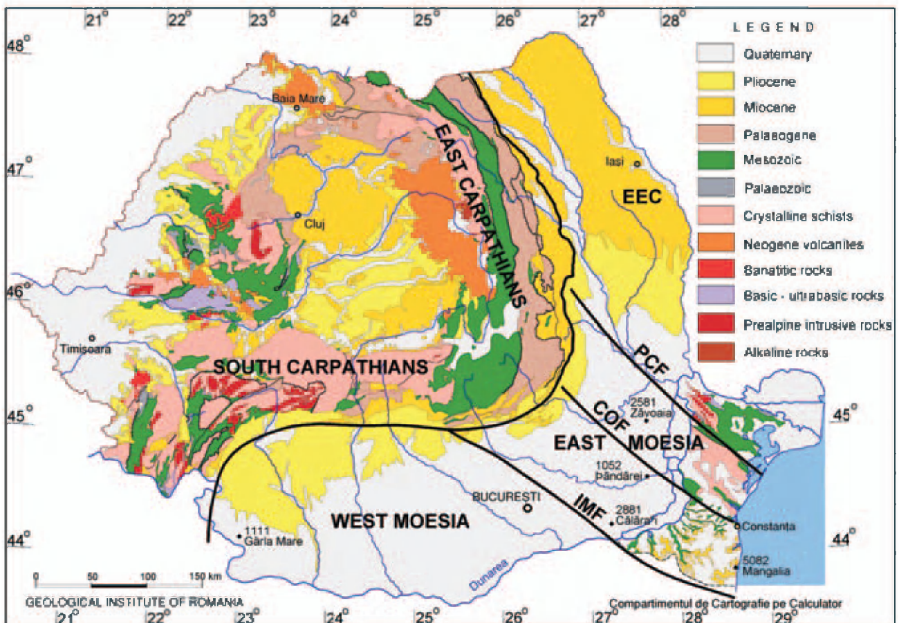
Figure 1. Schematic geological map of Romania with the location of the Moesian Platform and the larger tectonic units; the location of important boundary faults. Abbreviations: PCF-Peceneaga-Camena Fault; COF-Capidava-Ovidiu Fault; IMF-Intra-Moesian Fault; EEC-East European Craton.
