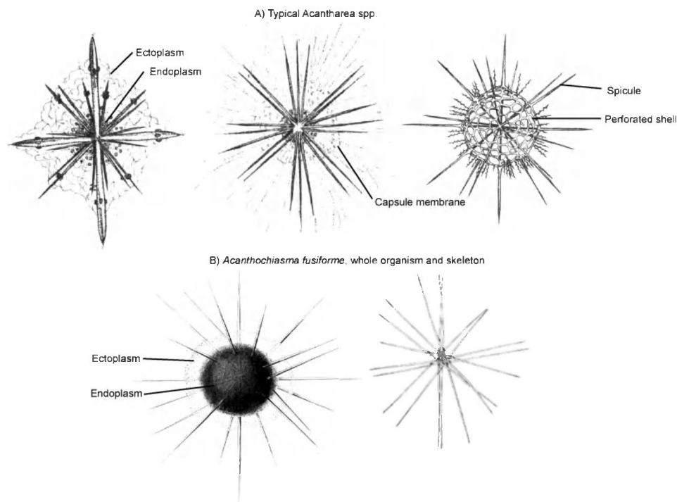
Fig. 1. Acanthareans (from Schewiakoff, 1926).
