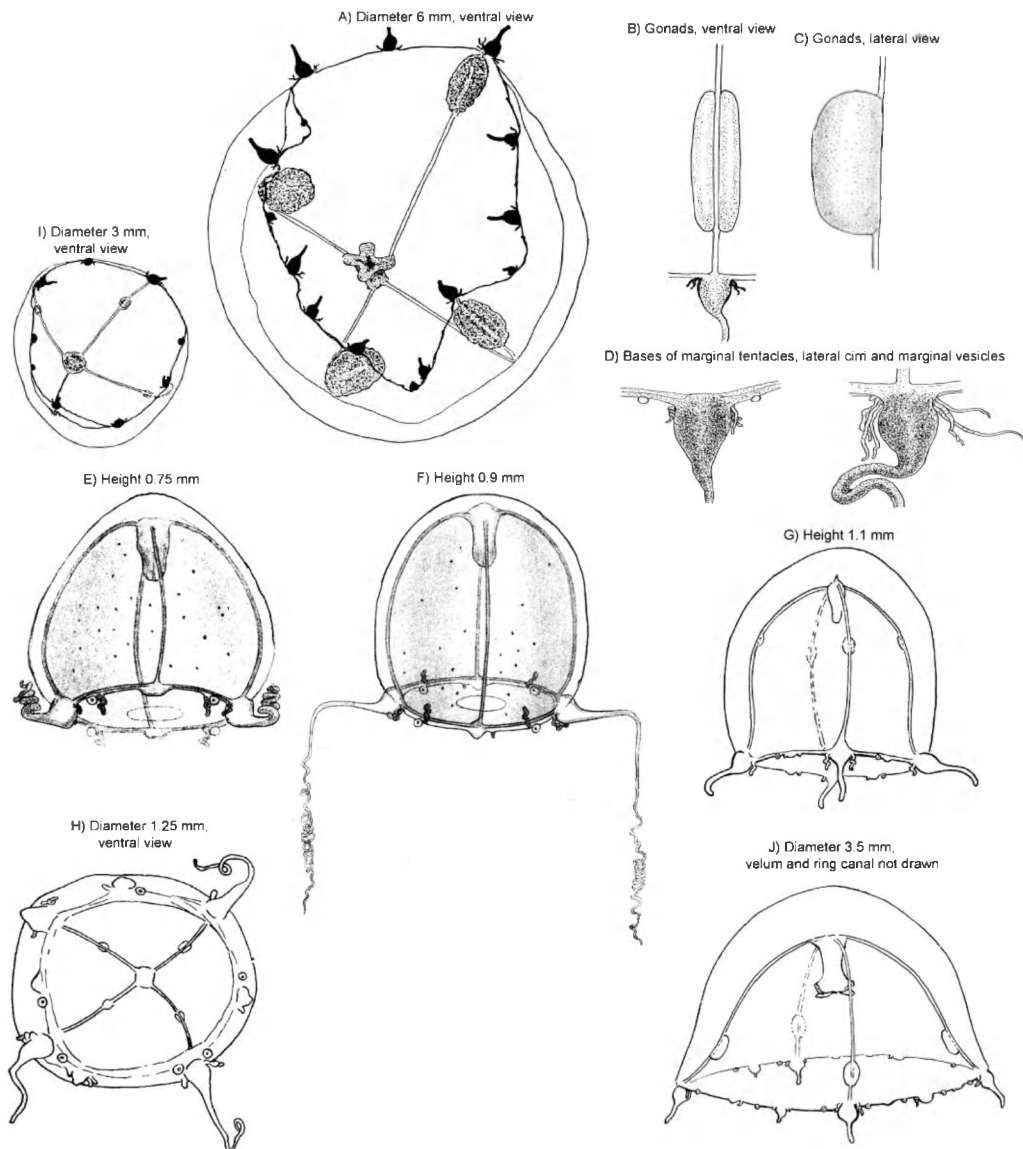
Fig. 61. Lovenella clausa (A-F, I from Russell, 1953; G, H, J from Russell, 1936, as Eucheilota hartlaubii ).
