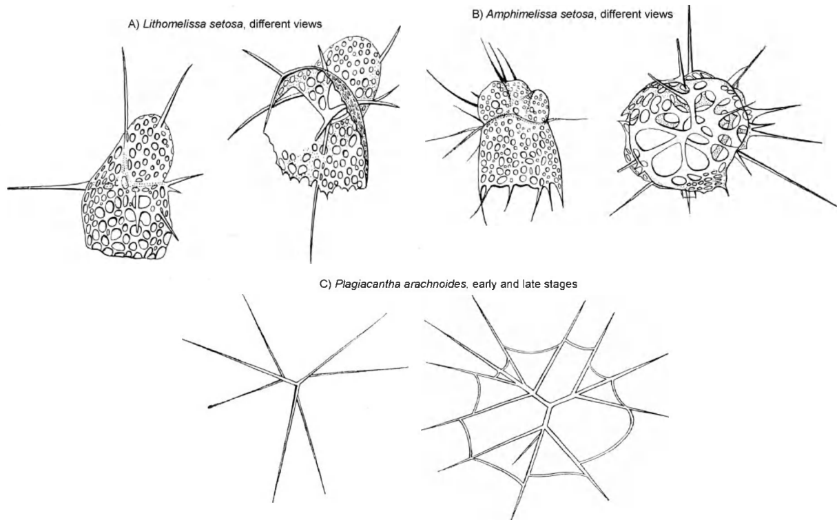
Fig. 2. Skeletons of Polycystinea species recorded at Plymouth (from Schröder, 1914).
