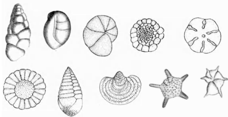
Fig. 1. Examples of benthic foraminiferans (from Cushman, 1928).
