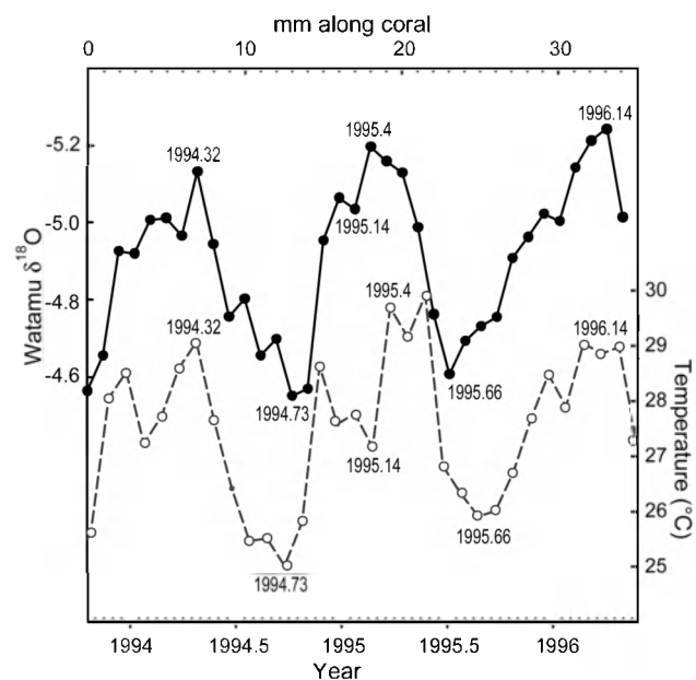
Fig. 2 Oxygen isotope ( \delta^{18}\text{O} ) profile versus depth in a coral core from Watamu for the most recent 2 years (upper – registered as a function of depth in mm) compared with GISST 3.2 ocean temperature data (lower – registered as a function of month/year). The dates on each curve are calendar age “pick points” for aligning the coral depth data with the monthly SST data in order to construct an optimized sub-annual age model.
