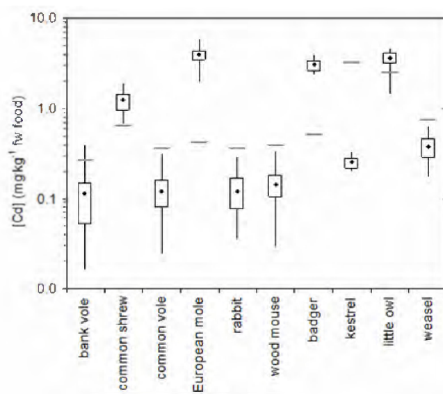
Fig. A-2.7: Predicted exposure concentrations ( \text{mg kg}^{-1} fresh wt food) of cadmium for 10 vertebrate species in the study area “Afferdensche en Deetsche Waarden”. Mean values are indicated by black diamonds; total range (minimum and maximum) are indicated by vertical lines; 10 th and 90 th percentiles are indicated by boxes; predicted no-effect concentrations ( \text{mg kg}^{-1} fresh wt food) are represented by grey horizontal line marks.
