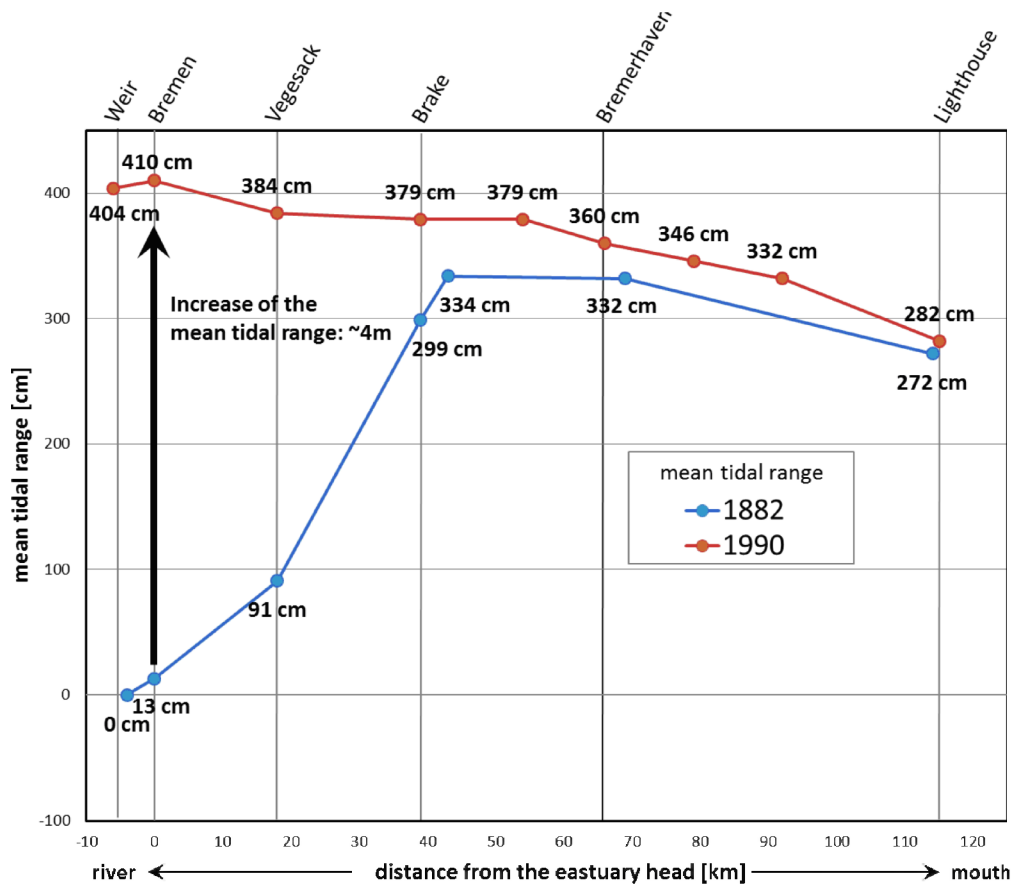
Fig. 5-1: Tidal wave development along the Weser
