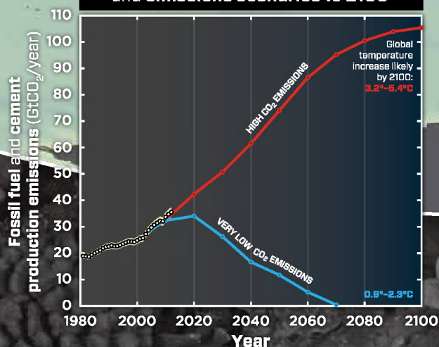
Observed CO 2 emissions and emissions scenarios to 2100
