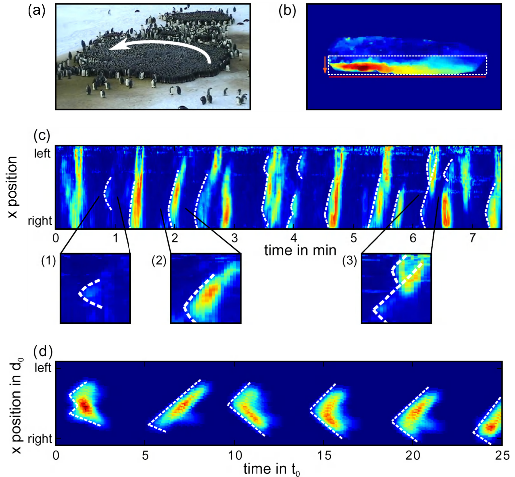
Figure 6. Optical flow analysis of the traveling wave dynamics. (a) Circular huddle with counter-clockwise (white arrow) rotational movements (copyright M Beaulieu and A Ancel, CNRS/IPEV). (b) Frame of the optical flow velocities in the huddle in (a). The flow velocity magnitude is column-wise averaged in the y -direction (orange arrow) over the lower half of the huddle (white dashed rectangle). The resulting line profile of the flow velocities along the x -direction (indicated by the red line) is plotted in the kymographs below. (c) The kymograph of the huddle movements during a 7 min period. White lines indicate wave fronts. Enlarged areas show (1) a decaying wave, (2) a non-decaying wave and (3) a merging event of two waves triggered at different positions. (d) Kymograph of the huddle movements in the simulation.
