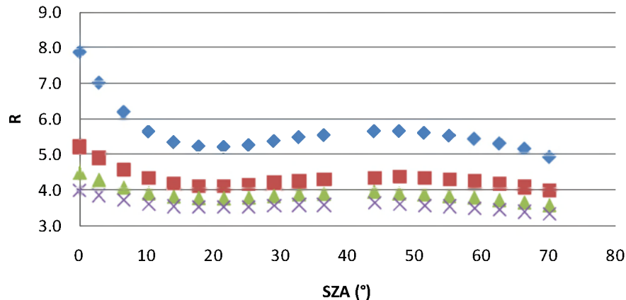
510 nm; 10 m/s
