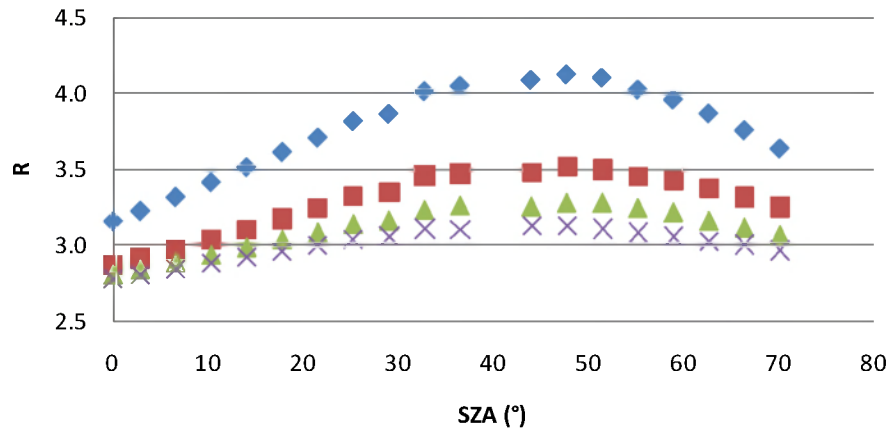
510 nm; 1 m/s
