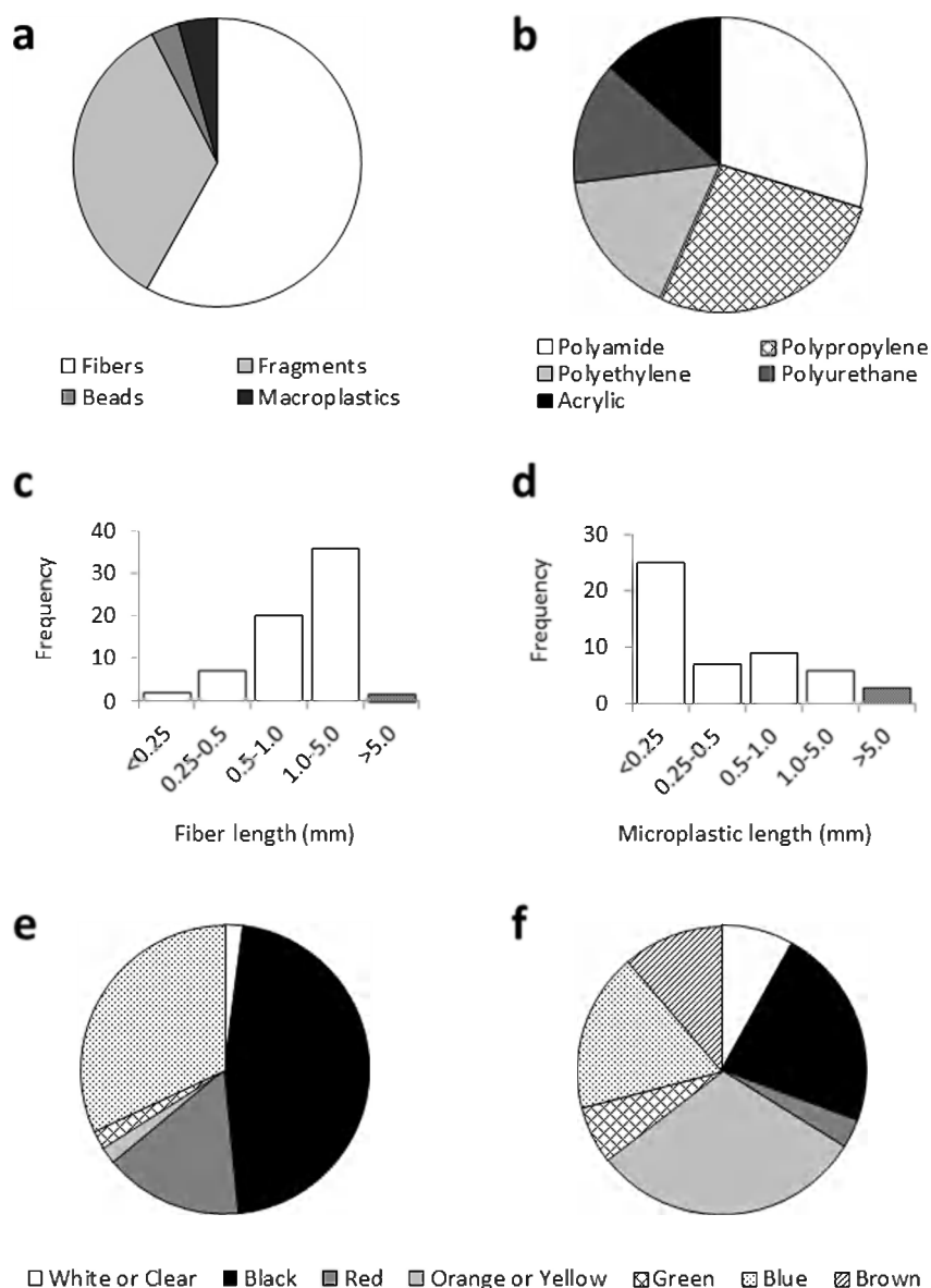
Figure 6 | Plastic litter extracted from two western English Channel sites varied by form, polymer, size and colour. (a) suspect debris was categorized as microplastic fibre, fragment or bead, or macroplastic ( >5 mm) ( n = 162 ); (b) FT-IR analysis was used to determine the constituent polymer of a sub-sample ( n = 40 ) of the suspected microplastic litter (note: 3 of these items were categorized as non-plastic, excluded from figure); sizing was conducted by either measuring (c) the length of a sub-sample of fibres ( n = 67 ), or (d) the widest diameter of a sub-sample of non-fibrous plastic litter present ( n = 50 ); colour was categorized for both (e) fibrous ( n = 97 ), and (f) non-fibrous litter ( n = 62 ) present.
