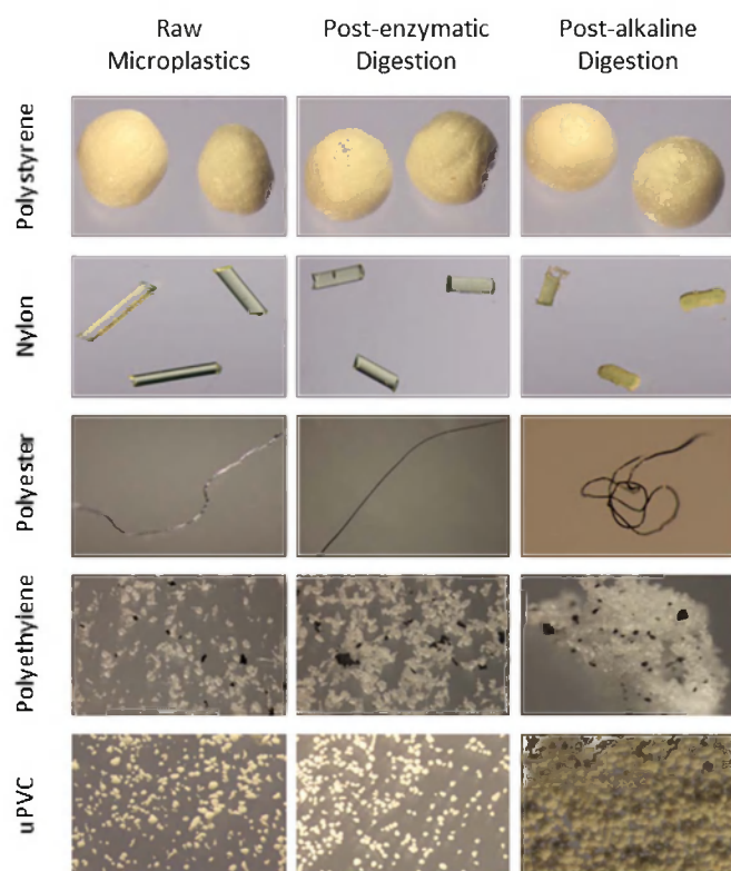
Figure 5 | Microplastics photographed before and after enzymatic and alkaline digestion. Alkaline hydrolysis resulted in structural damage to Nylon fibres, melding of polyethylene fragments and discoloration to uPVC granules. Magnification: polystyrene spheres x40; Nylon line x20; polyester fibre x63; polyethylene granules x200; uPVC powder x160.
