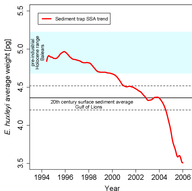
Figure 9. Comparison of sediment trap with sediment data. Emiliania huxleyi SSA trend in coccolith weight values from the sediment trap in the Gulf of Lions in comparison with sediments from a 20th century sediment surface (dashed lines indicating 95 % confidence interval), and a pre-industrial Holocene sediment record (blue shaded area indicating range of average weight values) from the NW Mediterranean.
