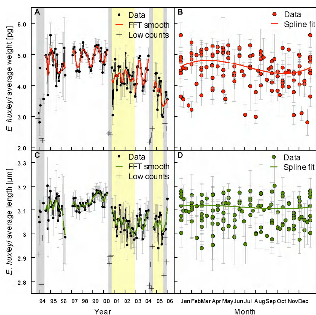
Figure 2. Emiliania huxleyi mean coccolith length and weight over the sediment trap deployment period (A, C) and on a composite year (B, D). Long-term trends, seasonal variability, periods with extremely low average weight (grey shade) and periods with reduced/changed seasonality (yellow shade) are shown.
