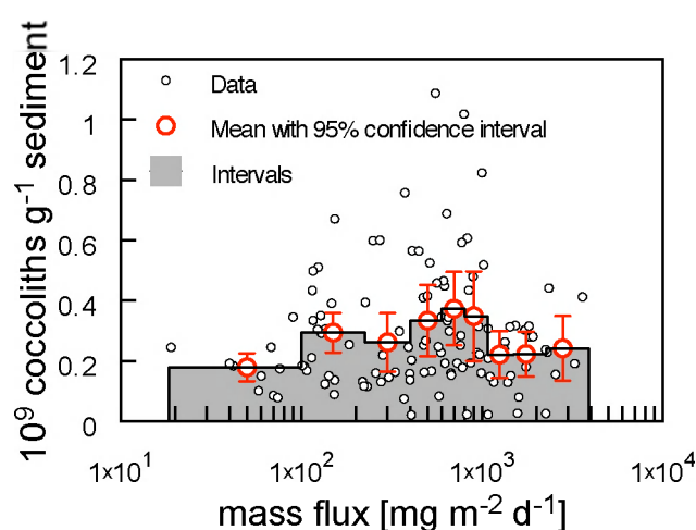
Figure 3. Emiliania huxleyi coccolith concentration in trap material versus total mass flux. Individual data points show an irregular scatter. Also the mean values within the mass flux intervals indicated by the grey bars show no increase with mass flux, indicating small influence of sediment transport and resuspension on coccolith concentration.
