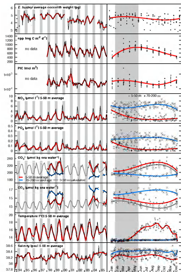
Figure 4. Emiliania huxleyi coccolith weight versus environmental data. Left: time period from 1993 to 2005 during which additional data was available. Thin lines represent original data. Bold colored lines are fast Fourier transform smoothed data. Right: data as on the left plotted on a composite year, indicating seasonal trends. Bold lines represent spline fits. Grey bars indicate the time period from February to May.
