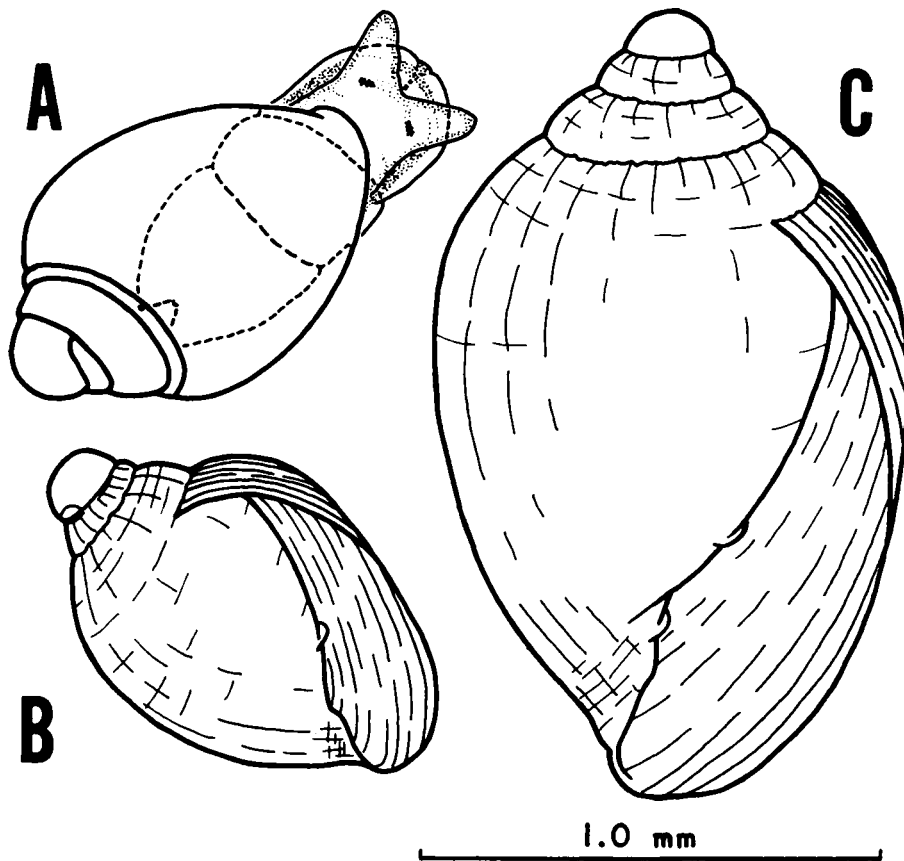
FIGURE 7. Later spat stages of Melampus : (A) dorsal view of a living specimen of a young spat about 4 to 5 weeks after settlement; (B) the dextral turbinat shell of a similar spat; and (C) shell of a spat about 8 weeks after settlement, in which the adult aperture shape (reflecting the growth gradients of the mantle-edge) is already established. Later shell growth is isometric, see text.
