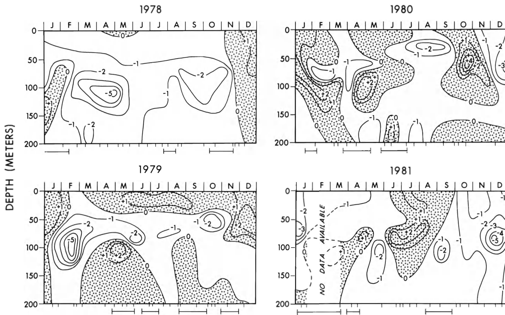
Figure 4 (cont.) Anomaly (°C) in bottom temperature.
