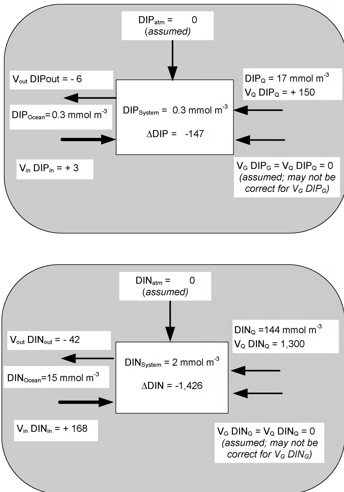
Figure 37. DIP and DIN budgets for Laguna de Terminos based on data for the wet period between June and January, but expressed as annual rates. See text for details of flux calculations. Fluxes in 10^6 \text{ mol year}^{-1} .
