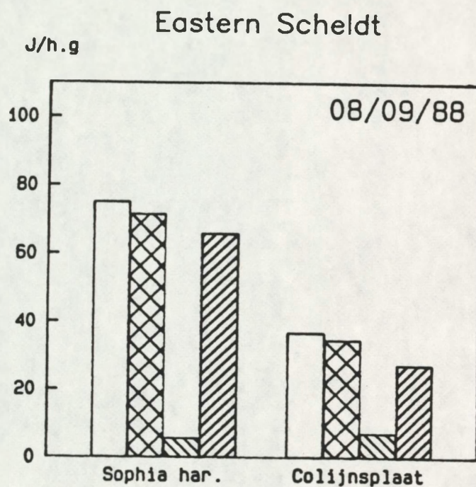
Figure 6. The SFG and its components measured in mussels exposed at Sophia-harbour and Colijnsplaat(yachtingharbour) at two different time intervals. Each bar represents the mean of 4 animals.
