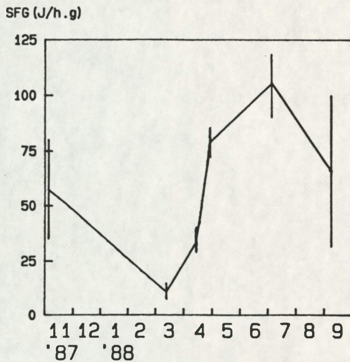
Figure 2. Annual cycle of the SFG of mussels exposed at Sophia-harbour, fieldstation, serves as reference site. Each point represents the mean of 4 animals, vertical bars indicate SD.
