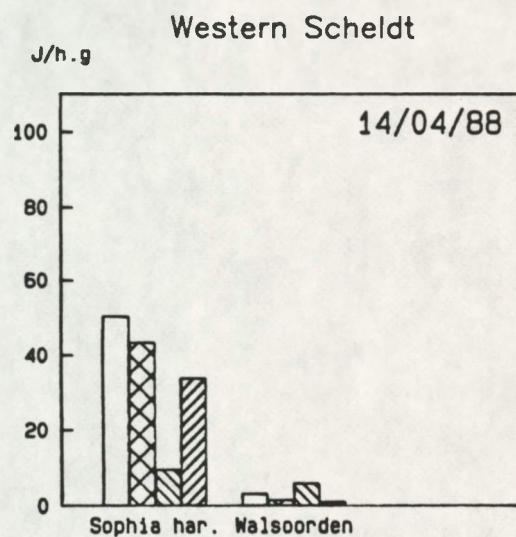
Figure 7. The SFG and its components measured in mussels exposed at Sophia-harbor and at the locations Vlissingen and Walsoorden in the Western Scheldt at three different exposure times. The cage exposed at Vlissingen was wash away after the first retrieval. Each bar represents the mean of 4 animals.
