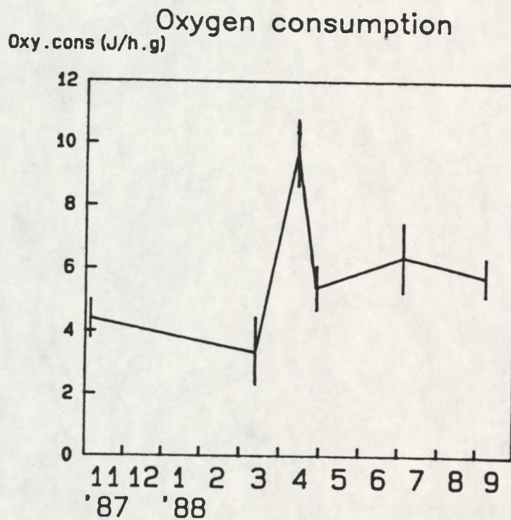
Figure 4. Annual cycle of the amount of energy absorbed(top) and oxygen consumption(bottom) of mussels exposed at Sophia-harbour, each point represents the mean of 4 animals, vertical bars indicate SD.
