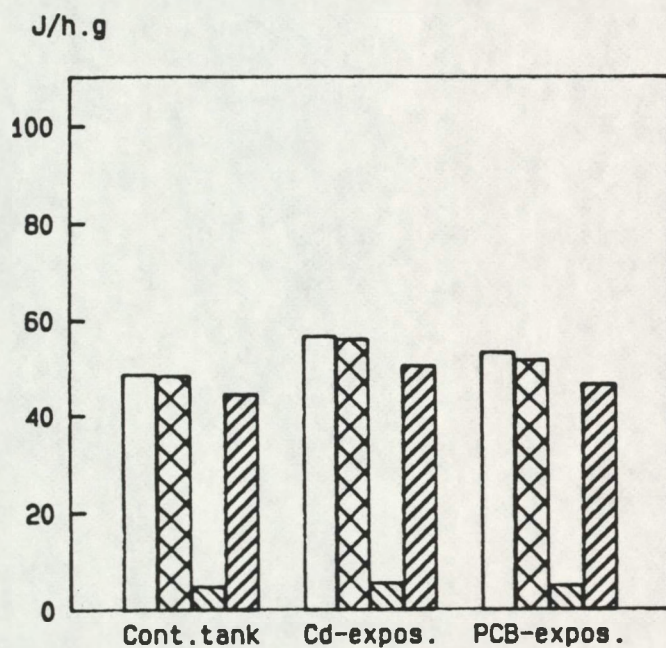
Figure 8. The SFG and its constituents determined with mussel exposed in an artificial exposure at the fieldstation. Mussels were exposed to 25 ppb cadmium and 0.5 ppb PCB for 10 and 11 weeks in two different experiments, top and bottom respectively. Each bar represents the mean of 4 mussels.
