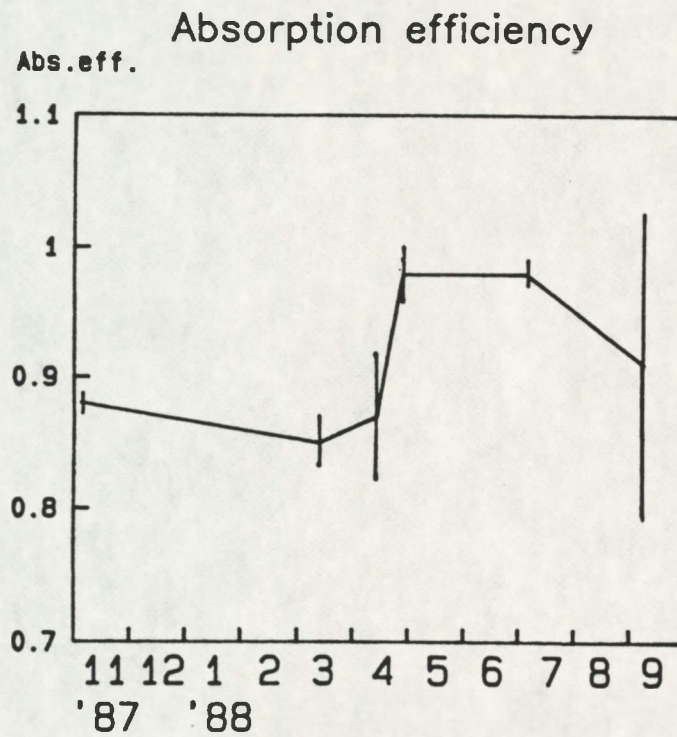
Figure 3. Annual cycle of the clearance rate(top) and absorption efficiency(bottom) of mussels exposed at Sophia-harbour, each point represents the mean of 4 mussels, vertical bars indicate SD.
