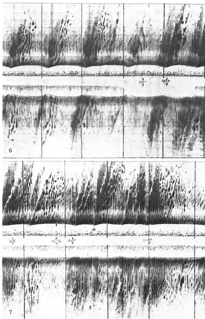
FIGURE 6. Side scan sonar record of symmetrical sandwaves on the col between the Sandettie and Fairy Banks.
