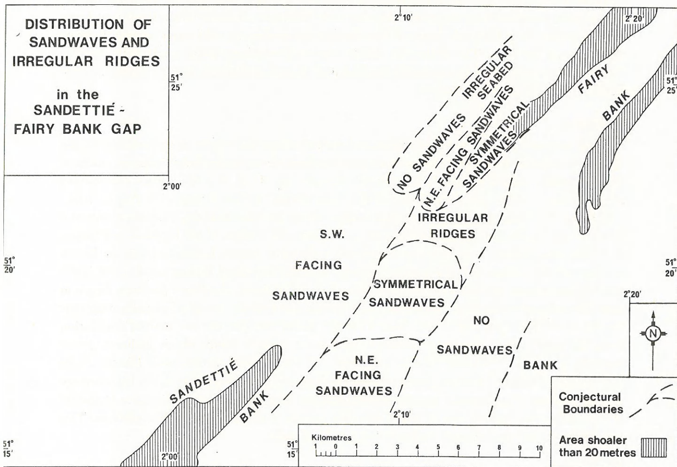
FIGURE 5. Distribution of sandwaves and irregular ridges in the Sandettie-Fairy Bank gap.
