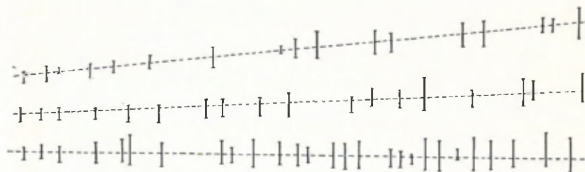
FIG. 7—Correlation of ranges of water planes suggesting differential upwarps of the land without evidence of eustatic changes of sea level.
