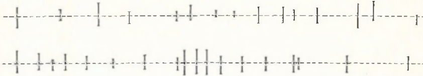
FIG. 5.—Correlation of maximum possible ranges (heavy vertical lines) of ancient water planes for different marine features, suggesting eustatic lowerings of sea level or uniform uplifts of a large crustal block.
