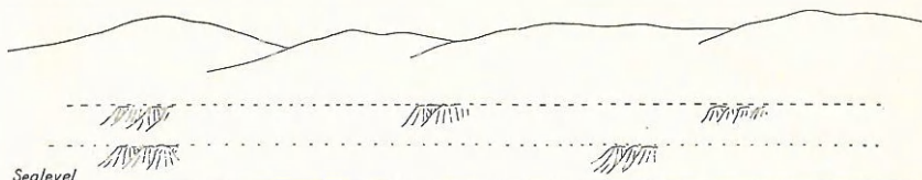
FIG. 3—Correlation of only part of the evidence of ancient marine levels here permits the inference that there are remnants of two horizontal elevated shore lines. Compare with Figure 4.
