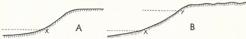
FIG. 1—Destructional terrace ( A ) and constructional terrace ( B ) compared.
