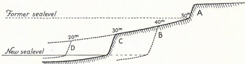
FIG. 2—Erosion terrace cut in former sea floor.
