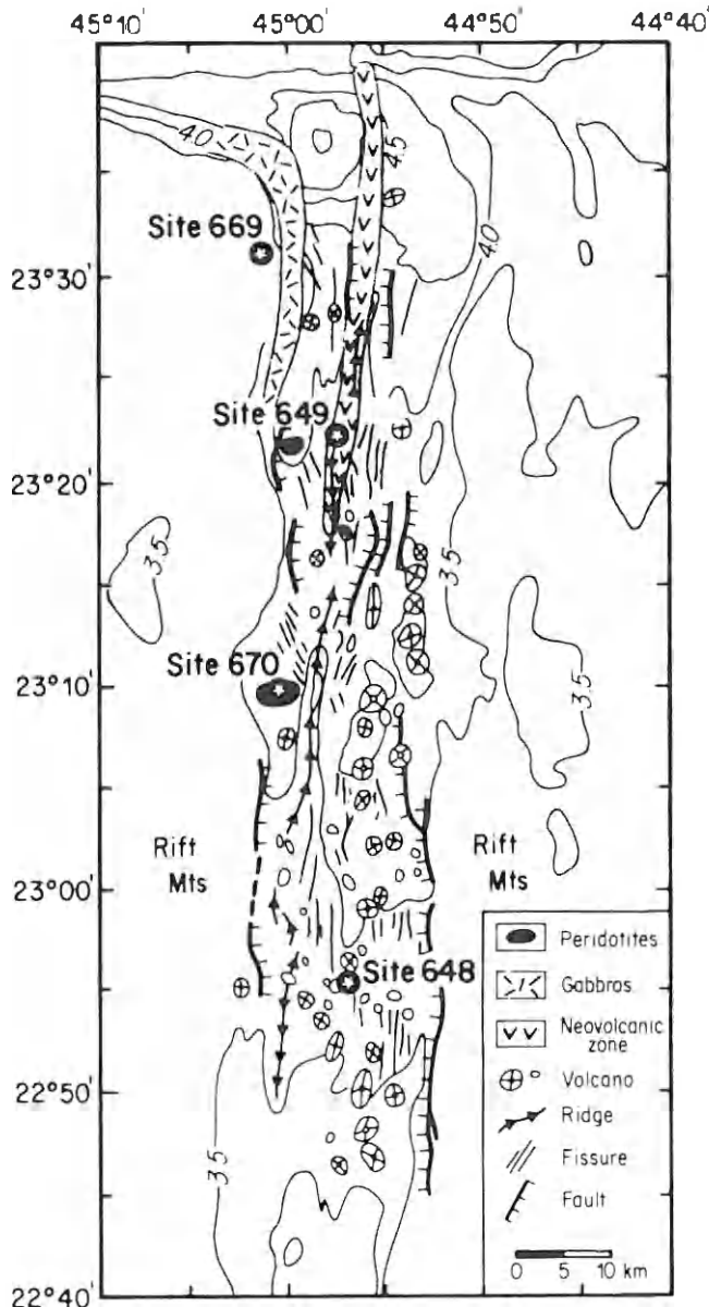
Figure 1. Geological and structural sketch map of the M.A.R. axial valley from 22°40'N (bottom) to the intersection with the Kane Fracture Zone (top). The main sites drilled during Legs 106 and 109 are indicated. Peridotite and gabbro outcrops and neovolcanic zones mainly after submersible surveys (Karson and Dick, 1983; Karson et al., 1987). Bathymetry and tectonic features from Detrick et al. (1985), Purdy and Detrick (1986), and Pockalny et al. (in press).
