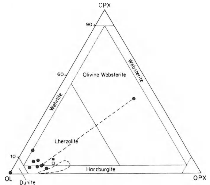
Figure 2. Serpentine-free compositions of the nine selected samples studied in this paper, plotted in the modal ternary ultramafic diagram. The collection consists of one dunite, four harzburgites, three lherzolites, and one olivine websterite. The cross indicates the calculated average composition of the whole sample set (see text). It is a cpx-poor four-phase lherzolite. The dashed line indicates the field of the North-Atlantic peridotites, after Michael and Bonatti (1985). Open square and black square = normative compositions of the Tinaquillo peridotite and pyrolite of Ringwood (1966), respectively (taken from Jacques and Green, 1980). The normative composition of the 8 kb melting point is from Takahashi and Kushiro (1983).
