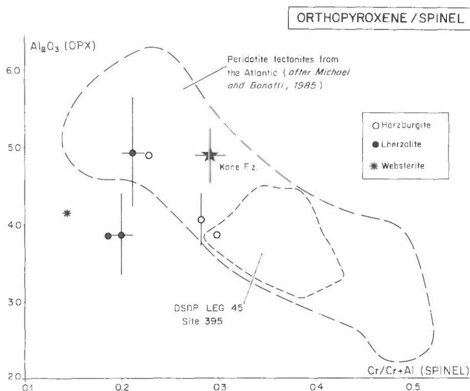
Figure 6. Diagram of the \text{Al}_2\text{O}_3 content (wt%) of the orthopyroxenes vs. the \text{Cr}/\text{Cr} + \text{Al} ratio of the spinels in the studied samples, and comparison with other data from the North Atlantic peridotites.
