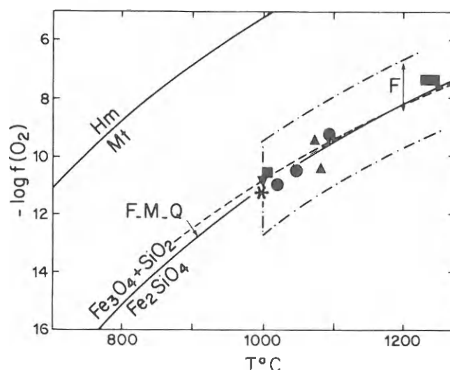
Figure 7. Oxygen fugacities calculated in the Site 670 peridotites for 10 kb pressure and at the blocking temperatures indicated by the olivine/spinel geothermometer (Table 6), close to 1000°C. The oxygen fugacities obtained for Site 670 peridotites, represented by the black inverted triangle (average of values given in Table 7), are compared with the fugacities calculated for some other oceanic peridotites (black circles = peridotites from ophiolitic massifs; other symbols = peridotite inclusions in alkali basalts).
