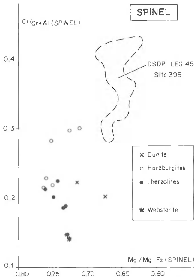
Figure 5. Diagram of the Cr/Cr + Al ratio (or Cr#) vs. the Mg/Mg + Fe ratio (or Mg#) in the spinels of the studied samples, and comparison with Site 395 data. A slight but significant difference appears in the Cr# between the harzburgites (average 24.2) and the lherzolites (average 20.6). The Cr# of the olivine websterite is clearly lower (14.4).
