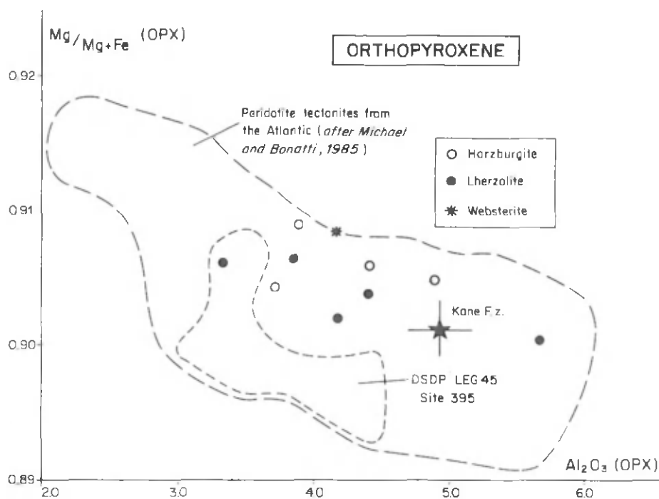
Figure 4. Diagram of the Mg/Mg + Fe ratio vs. the \text{Al}_2\text{O}_3 content (wt%) in the orthopyroxenes of the studied samples, and comparison with other data from the North Atlantic area (after Michael and Bonatti, 1985).
