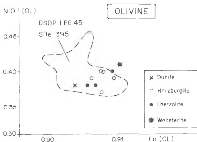
Figure 3. Diagram of the NiO content vs. Fo% of olivine in the studied samples, and comparison with Site 395 data.
