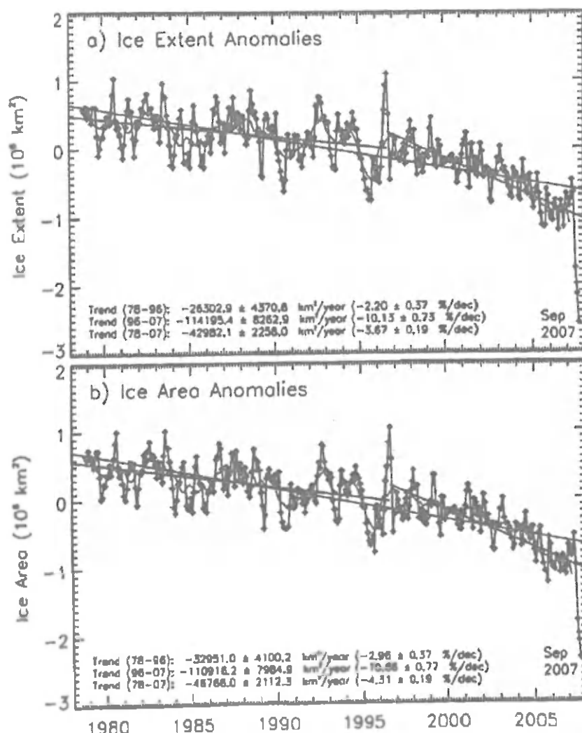
Figure 4. Monthly ice extent and ice area anomalies from November 1978 to September 2007 (green and blue), with the 12-month running average (red) and linear trend lines for the full record (black) and for 1978–1996 (green) and 1996–2007 (blue).
