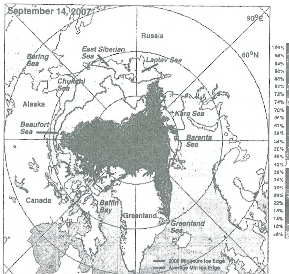
Figure 2. Daily Arctic ice concentrations from AMSR-E for 14 September 2007, when the ice cover reached its minimum extent. The gold contour represents the ice edge inferred from the average of the ice concentration maps during ice minimum extent over the period 1979–2006, while the red contour represents the ice edge during ice minimum in 2005, which was the previous record low.
