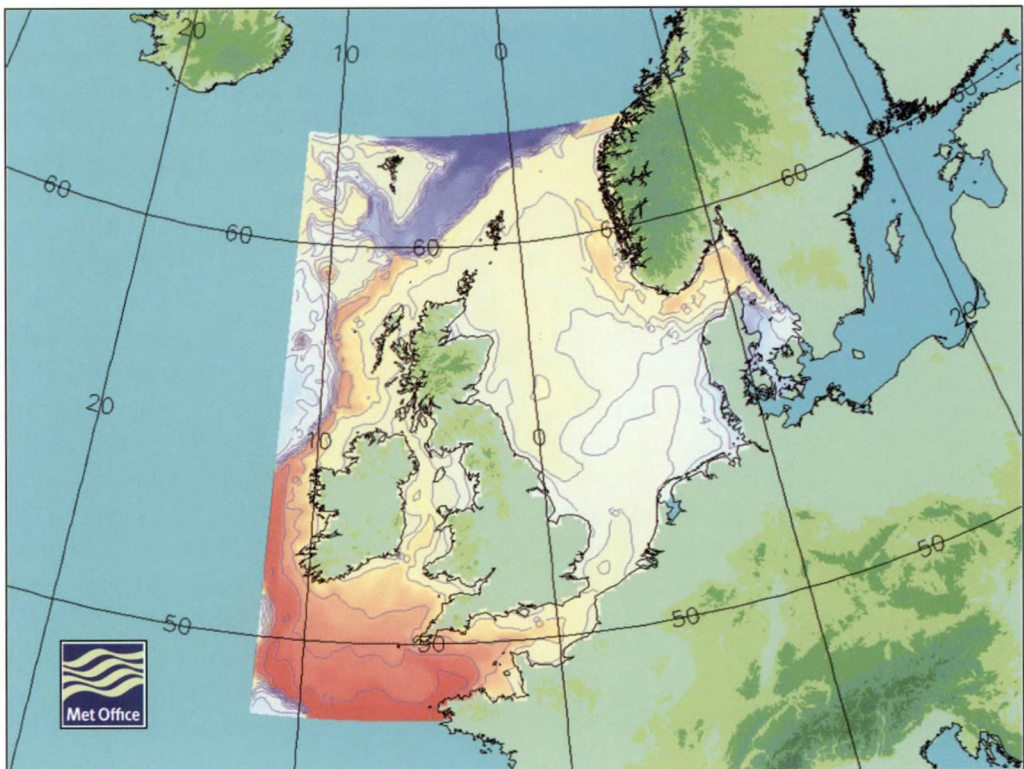
Figure 1.3 Shelf seas model on HORACE. Bottom temperature 5/3/2001
