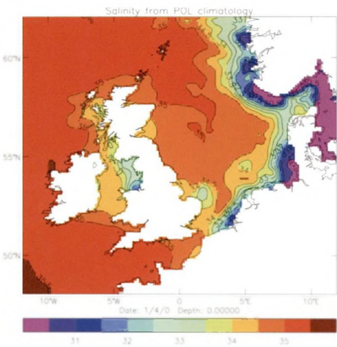
Figure 8 Salinity Climatology for April
