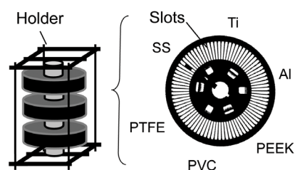
Figure 1 | Set-up used for biofilm development in and adjacent to a brine pool near the Thuwal cold seeps. The samplers contained six types of substrate for biofilm development, including aluminum (Al), polyether ether ketone (PEEK), Polyvinyl chloride (PVC), polytetrafluoroethene (PTFE), stainless steel (SS) and titanium (Ti). Material pieces were embedded in the slots of the carousel. Three containers were fixed in the frame and then immersed in the water.
