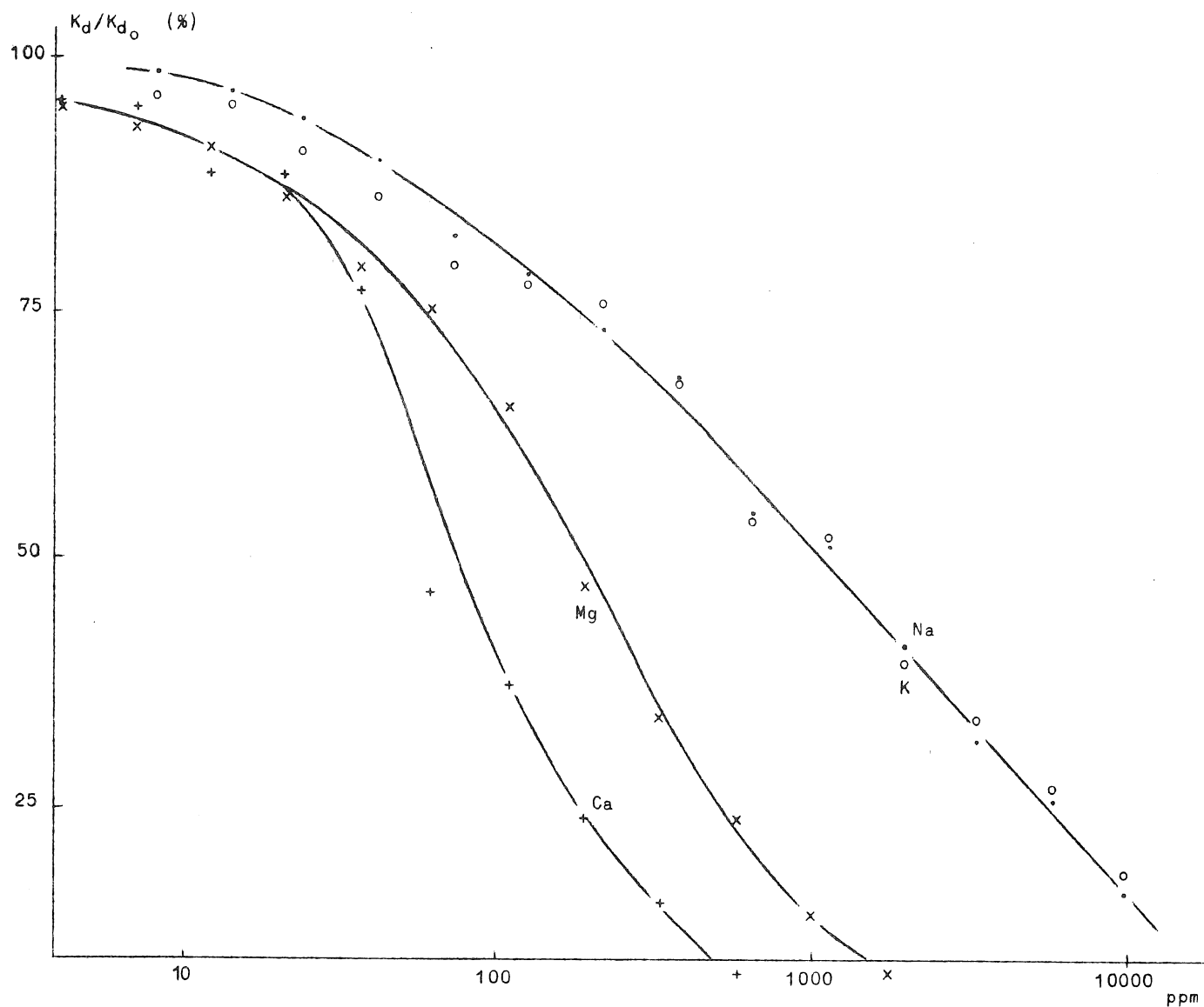
fig. 18. Cd^{109} Sorption versus competing cation concentration
