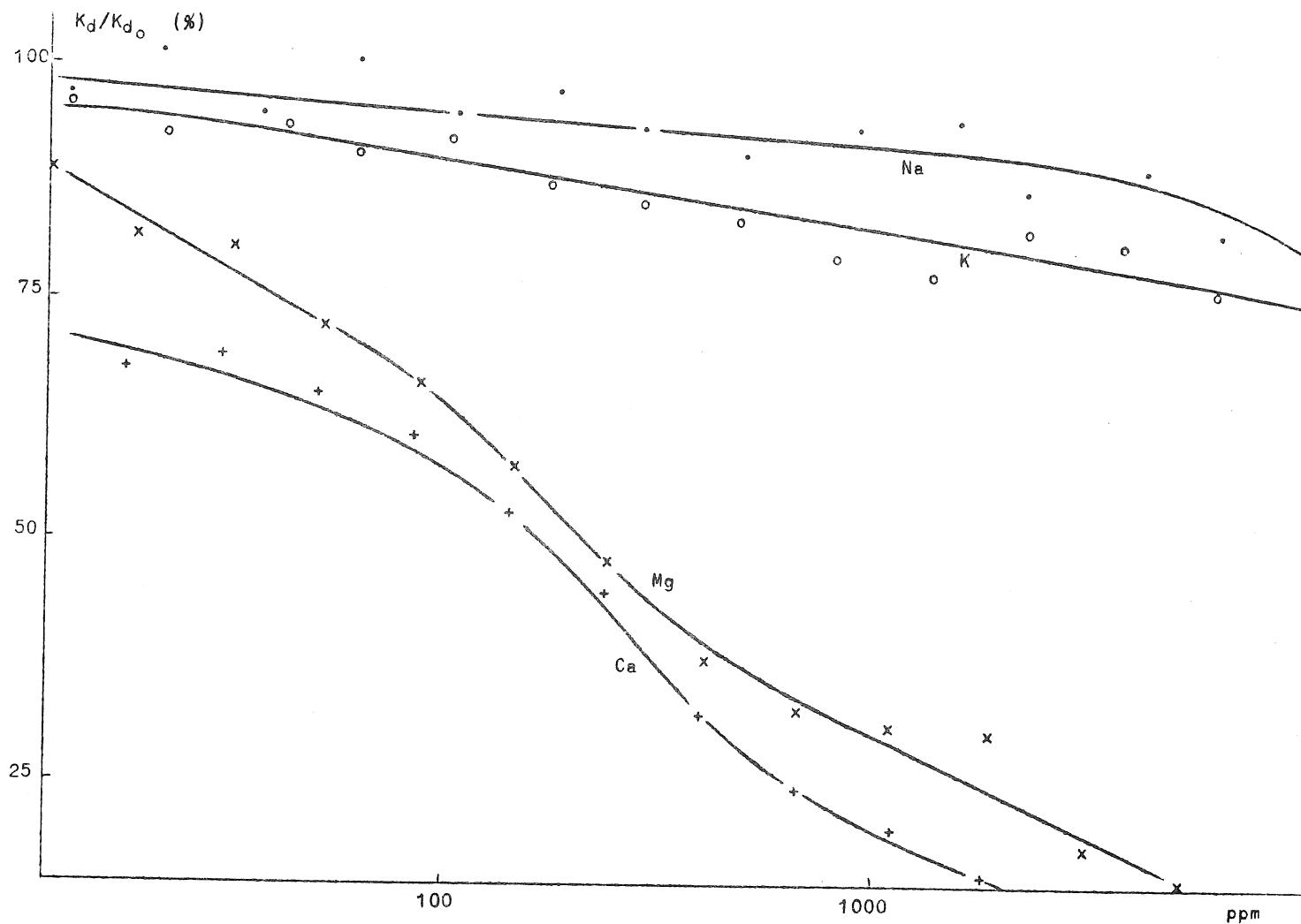
fig. 19. Mn 54 Sorption versus competing cation concentration
