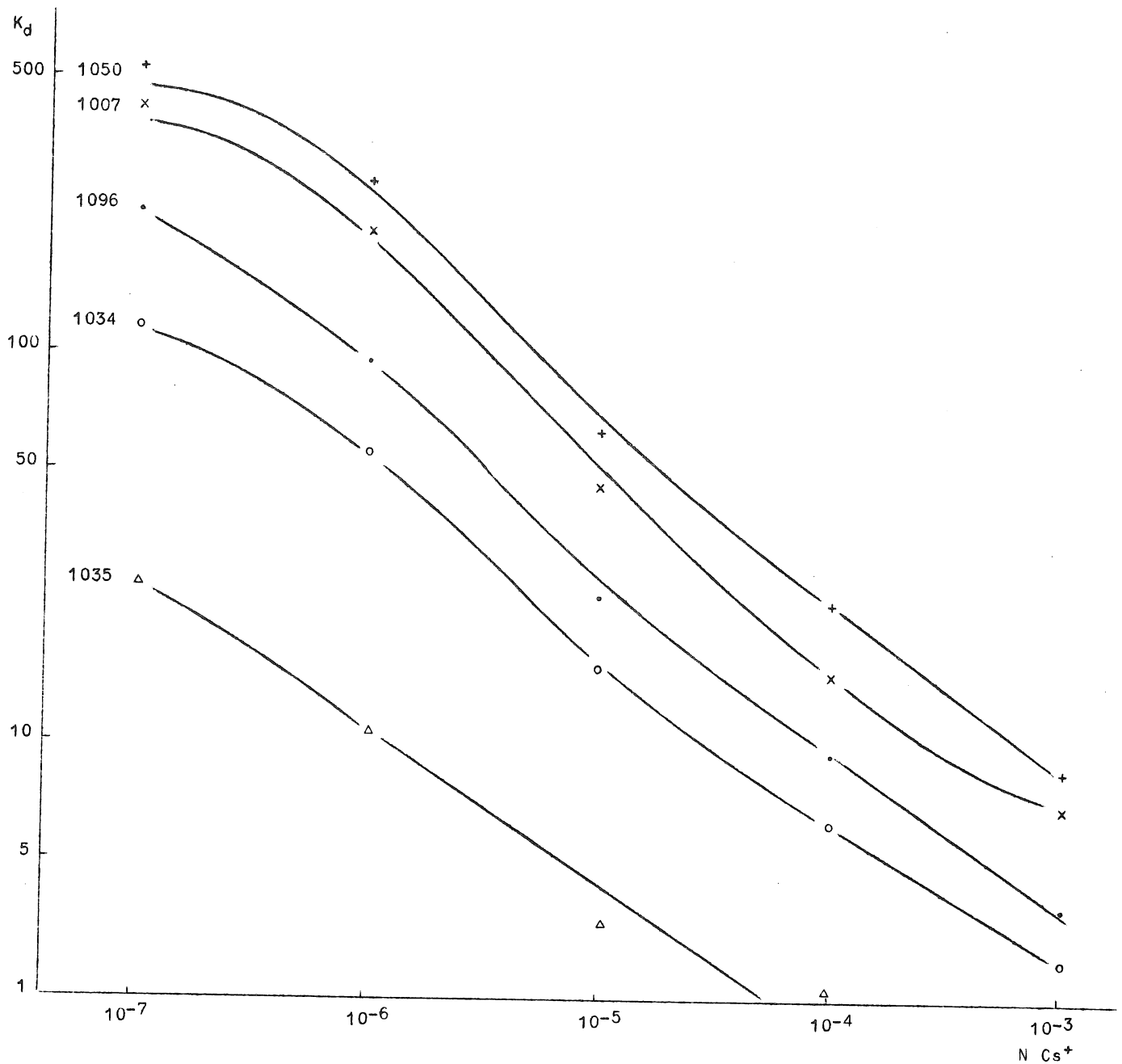
fig. 24. Cs 137 Sorption versus Cs concentration
