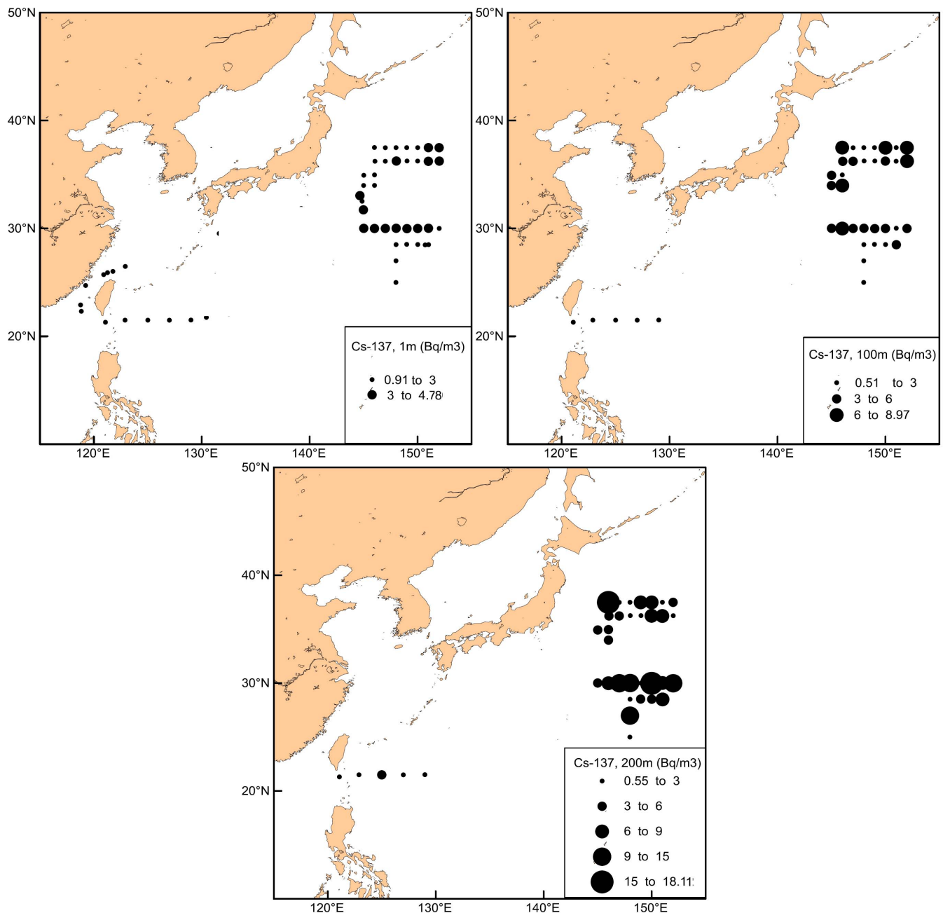
Figure 3 | The distributions of ^{137}\text{Cs} at depths of 1 m, 100 m and 200 m in the North Pacific. These figures were drawn using Surfer.
