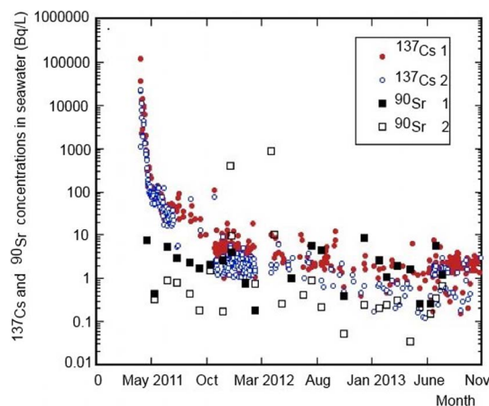
Figure 1 | Temporal variations of ^{137}\text{Cs} and ^{90}\text{Sr} activity concentrations in surface waters near the north (1) and south (2) water outlets (data from Refs. 4–7, 10–12, 15, 27–29). Relative data uncertainties (at 1 sigma) are below 10%.
