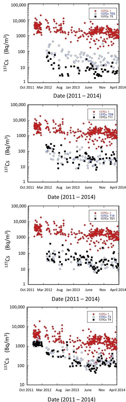
Figure 2 | Temporal changes of ^{137}\text{Cs} activity concentrations in surface waters at monitoring sites within 20 km from the Fukushima Dai-ichi NPP (data from Refs. 5–7, 14, 21). Notice remarkable differences between ^{137}\text{Cs} levels observed close to the FDNPP (St. 1, red dots) and the more distant stations. Relative data uncertainties (at 1 sigma) are below 10%. Positions of monitoring sites are given in Table 1.
