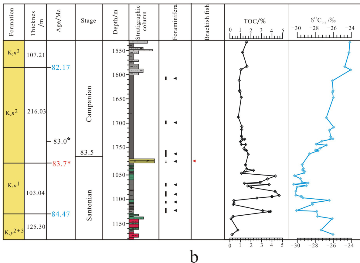
Figure 2 | Stratigraphic distributions of TOC and \delta^{13}C_{org} . (a): for Qingshankou Formation; (b): for Member 1 and Member 2 of the Nenjiang Formation. ◀ indicates the distribution of Foraminifera (Ref. 2) and ▶ indicates the distribution of brackish fish (Ref. 3).
