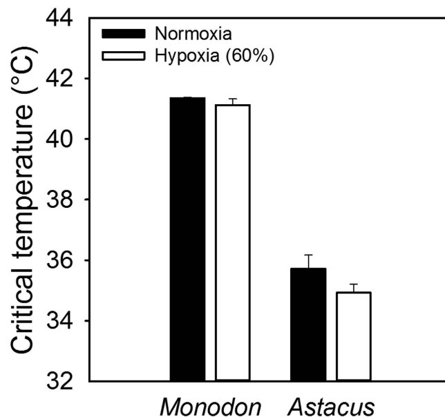
Figure 3. T_{crit} (°C) was unaffected by reduced oxygen tension (Normoxia and 60% air saturation) in the Giant tiger shrimp ( Penaeus Monodon ) ( n=8 ) ( P=0.798 ) and the European crayfish ( Astacus astacus ) ( n=9 ) ( P=0.052 ). Columns show means \pm SEM.
