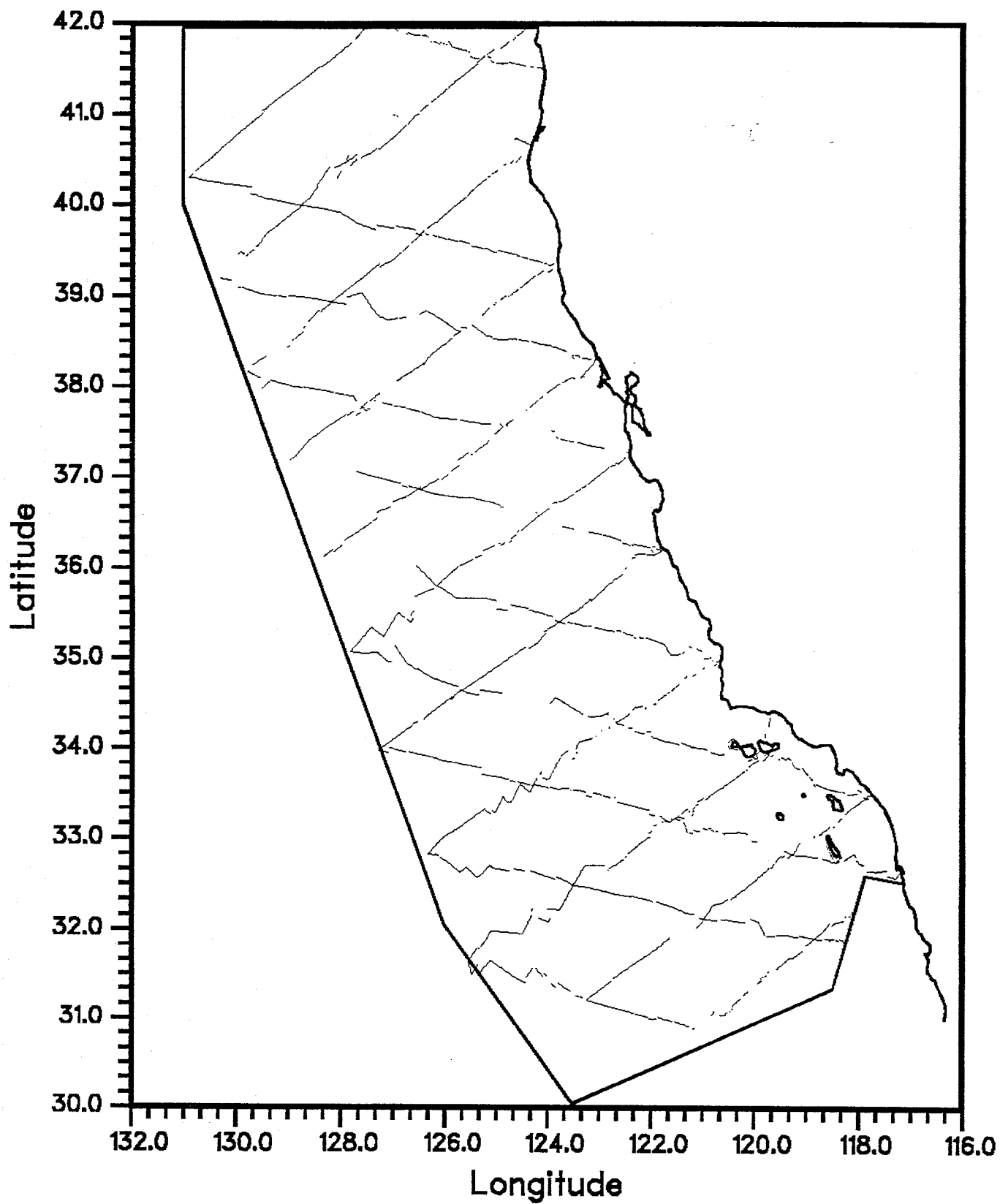
Figure 4. Tracklines surveyed during the 1991 CAMMS cruise.
