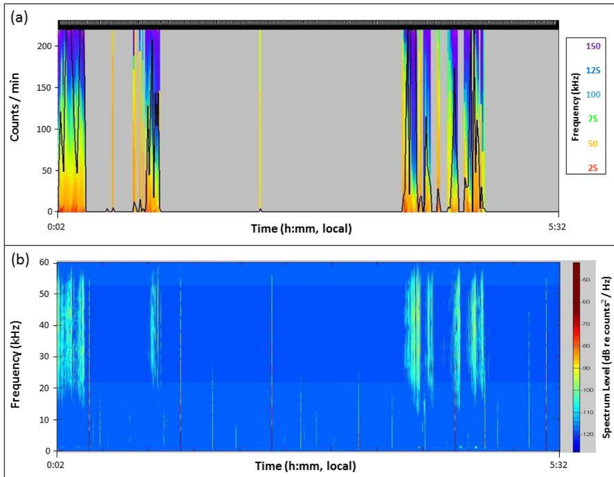
Figure 3.6. Representation of simultaneous recordings made on 7 February 2011 in Stone Bay from (a) C-POD and (b) DMON. (a) The C-POD recording is displayed using the manufacturer's software, CPOD.exe (Chelonia Ltd, UK) and showing Detected Positive Minutes (DPMs) of bottlenose dolphin echolocation. For each DPM, counts of clicks per minute in one-minute bins of quality categories Hi, Moderate and Low detections are shown, with color representing the frequency of clicks. (b) The DMON recording is displayed using Triton v. 1.64 (Scripps Institute of Oceanography, CA, USA) as a LTSA (Long Terms Spectral Average) showing several bouts of bottlenose dolphin echolocation.
