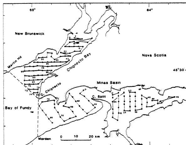
Fig. 1. Map of the upper Bay of Fundy showing the cruise tracks in Chignecto Bay and Minas Basin.
