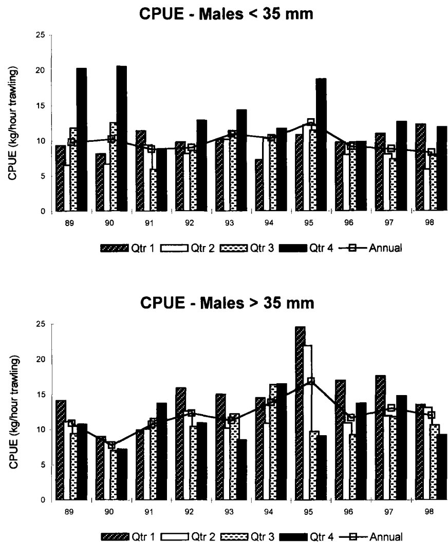
Figure 5.11.15. - South Minch (FU 12): CPUEs by sex and quarter, for selected size groups.
