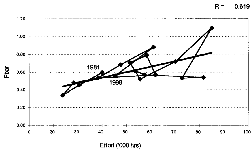
Figure 5.3.9. - Moray Firth (FU 9): Effort and Fbar, and relationship between them, for males and females.
