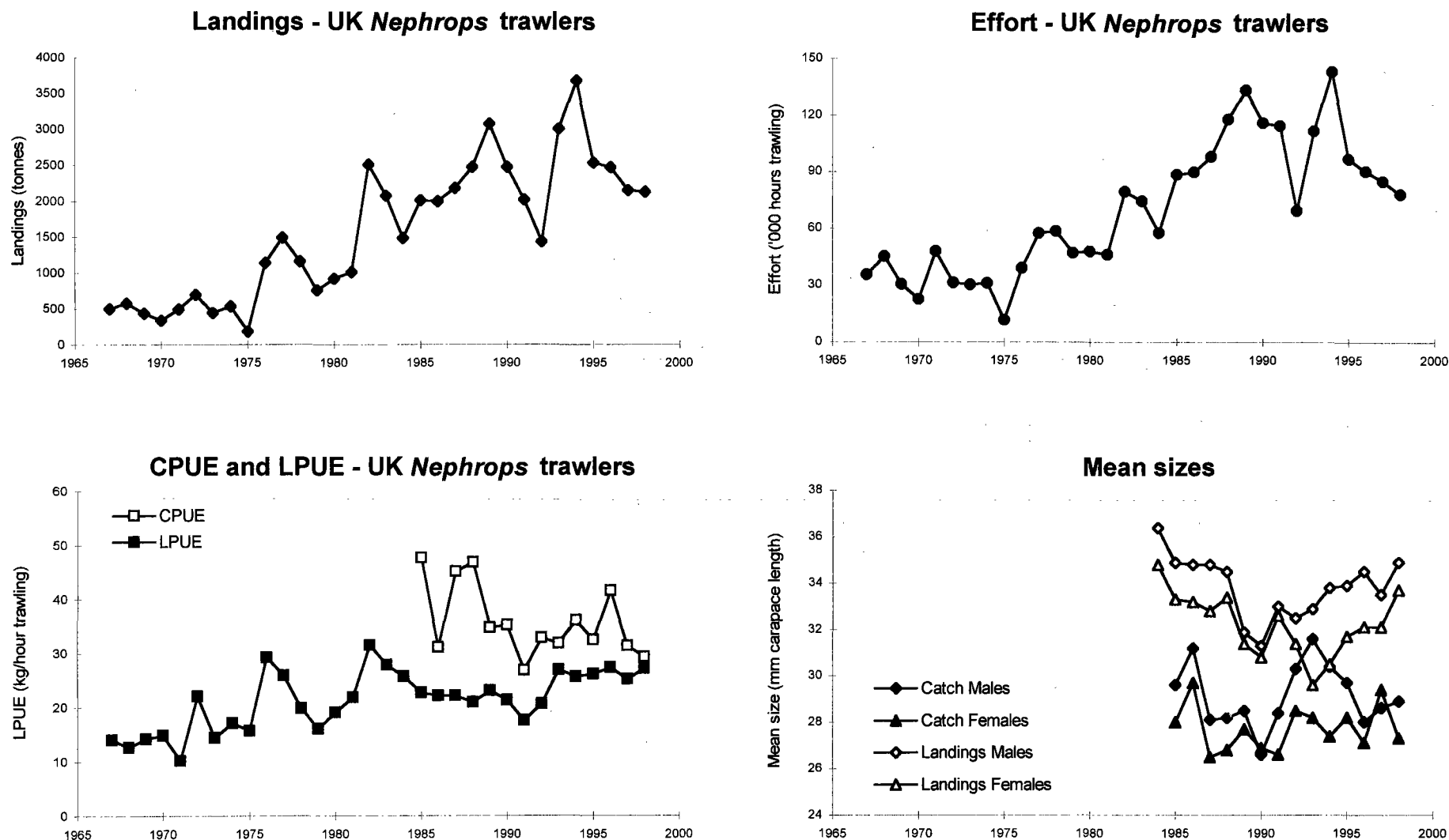
Figure 5.6.1. - Farn Deep (FU 6): Long-term trends in landings, effort, CPUEs, LPUEs and mean sizes of Nephrops in catches and landings.
