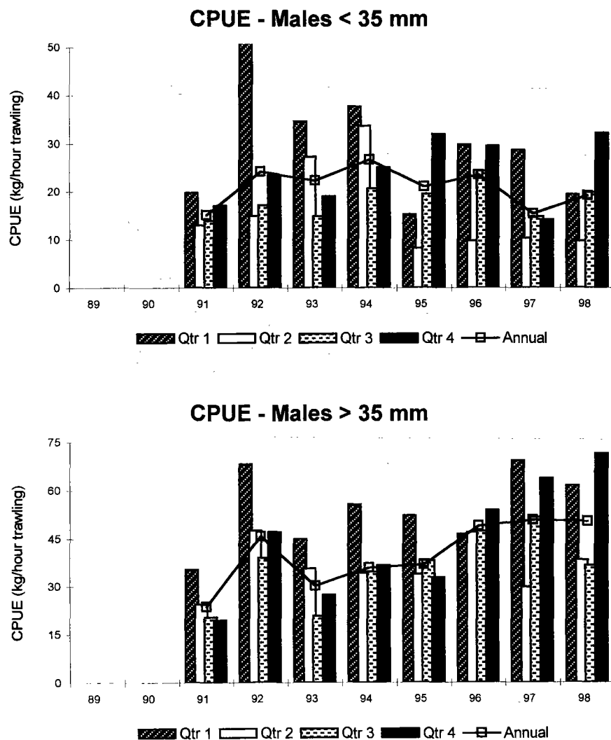
Figure 5.4.3. - Fladen (FU 7): CPUEs by sex and quarter, for selected size groups.
