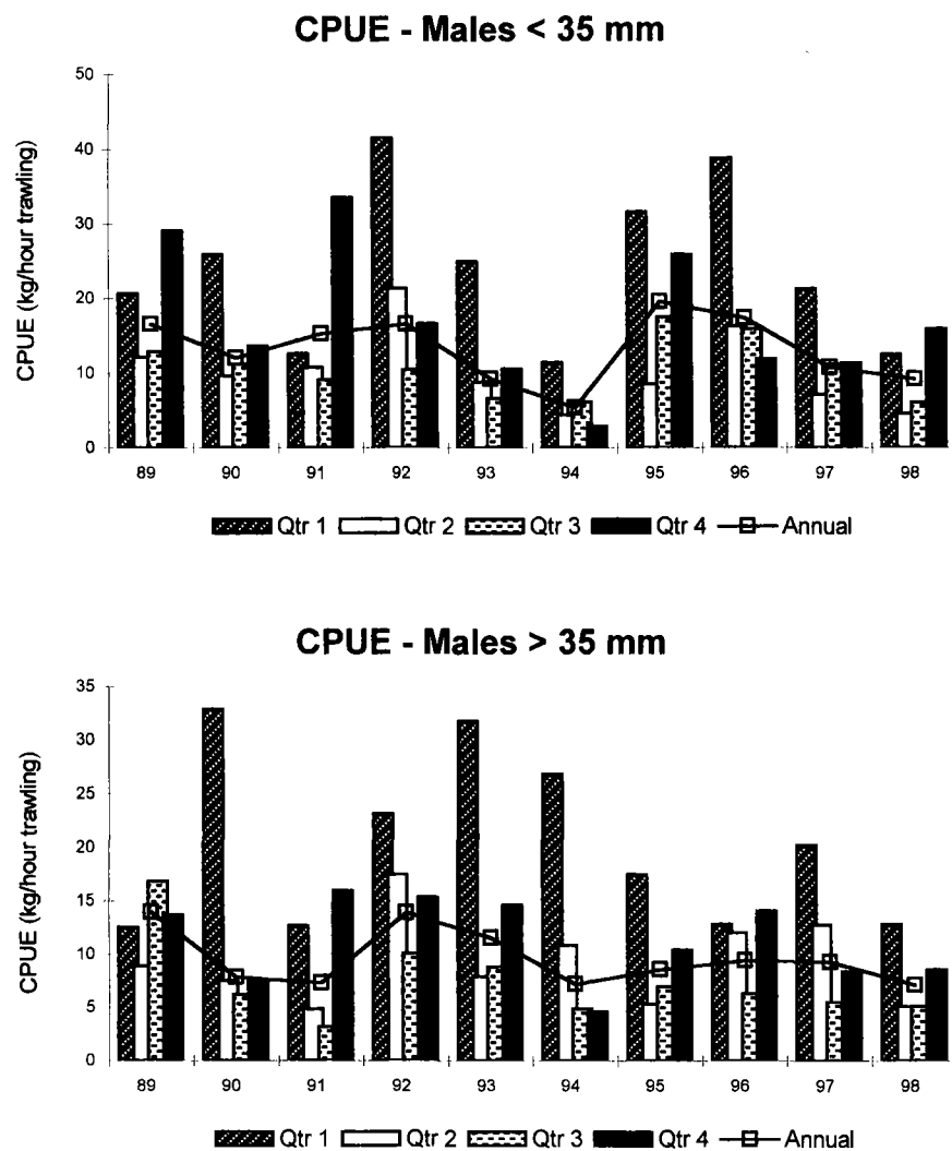
Figure 5.3.3. - Moray Firth (FU 9): CPUEs by sex and quarter, for selected size groups.
