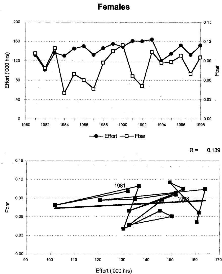
Figure 5.11.28. - Firth of Clyde (FU 13): Effort and Fbar, and relationship between them, for males and females.
