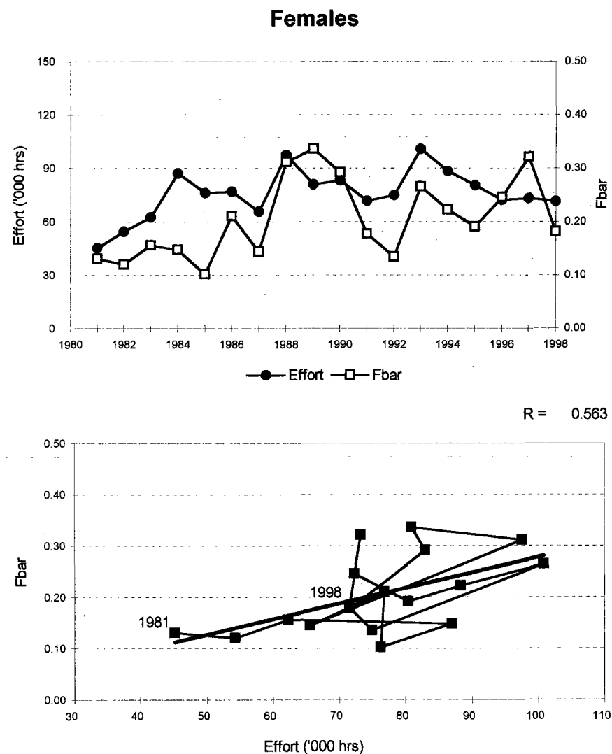
Figure 5.6.17. - Firth of Forth (FU 8): Effort and Fbar, and relationship between them, for males and females.
