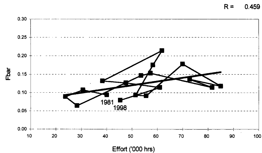
Figure 5.3.9. - Moray Firth (FU 9): Effort and Fbar, and relationship between them, for males and females.
