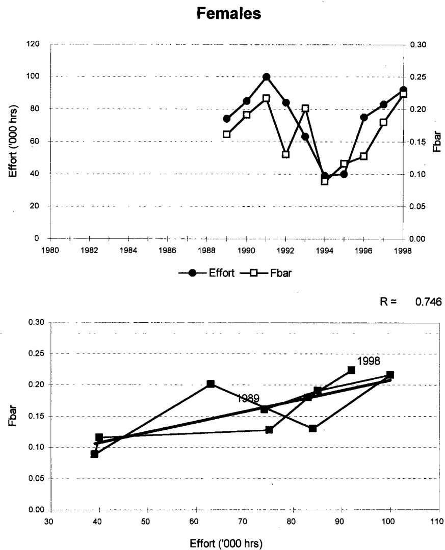
Figure 5.7.8. - Botney Gut - Silver Pit (FU 5): Effort and Fbar, and relationship between them, for males and females.
