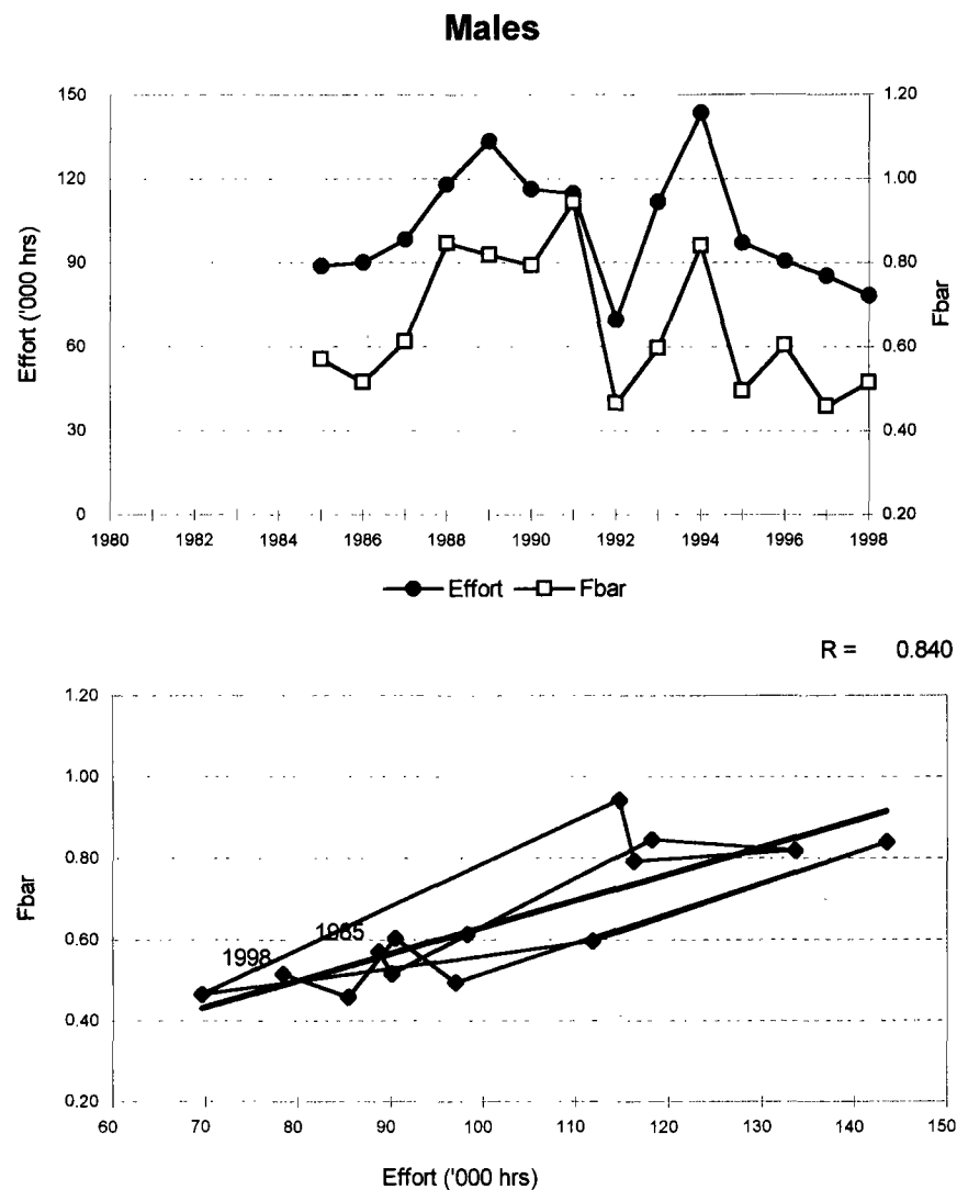
Figure 5.6.8. - Farn Deepes (FU 6): Effort and Fbar, and relationship between them, for males and females.
