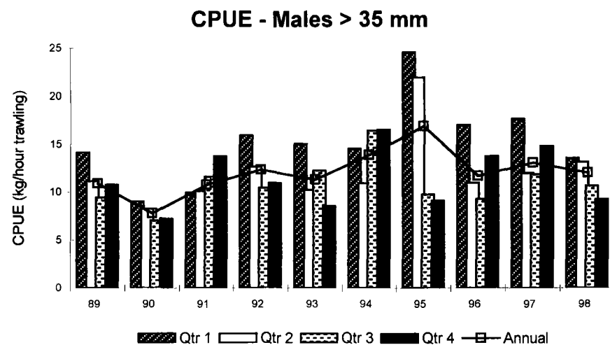
Figure 5.11.15. - South Minch (FU 12): CPUEs by sex and quarter, for selected size groups.
