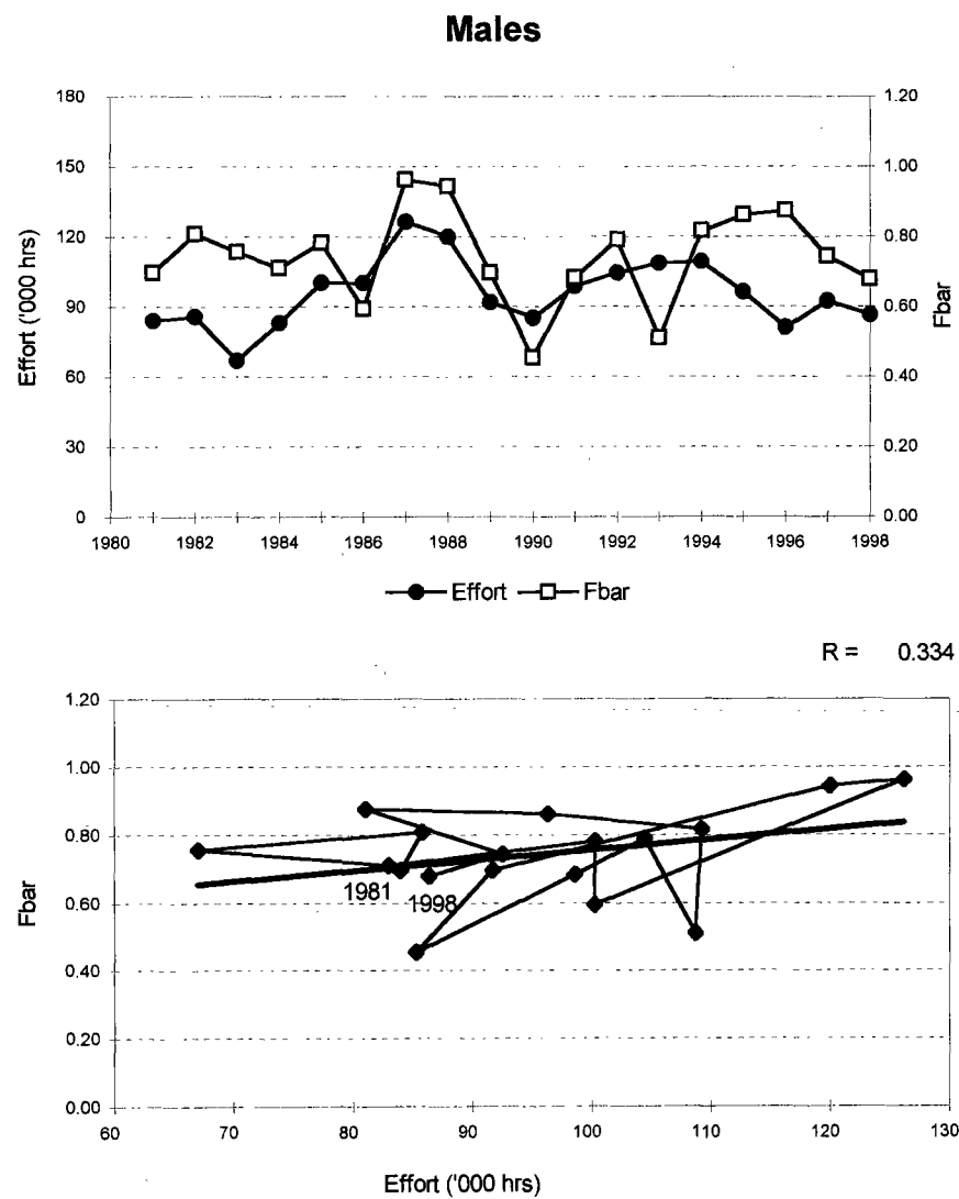
Figure 5.11.10. - North Minch (FU 11): Effort and Fbar, and relationship between them, for males and females.
