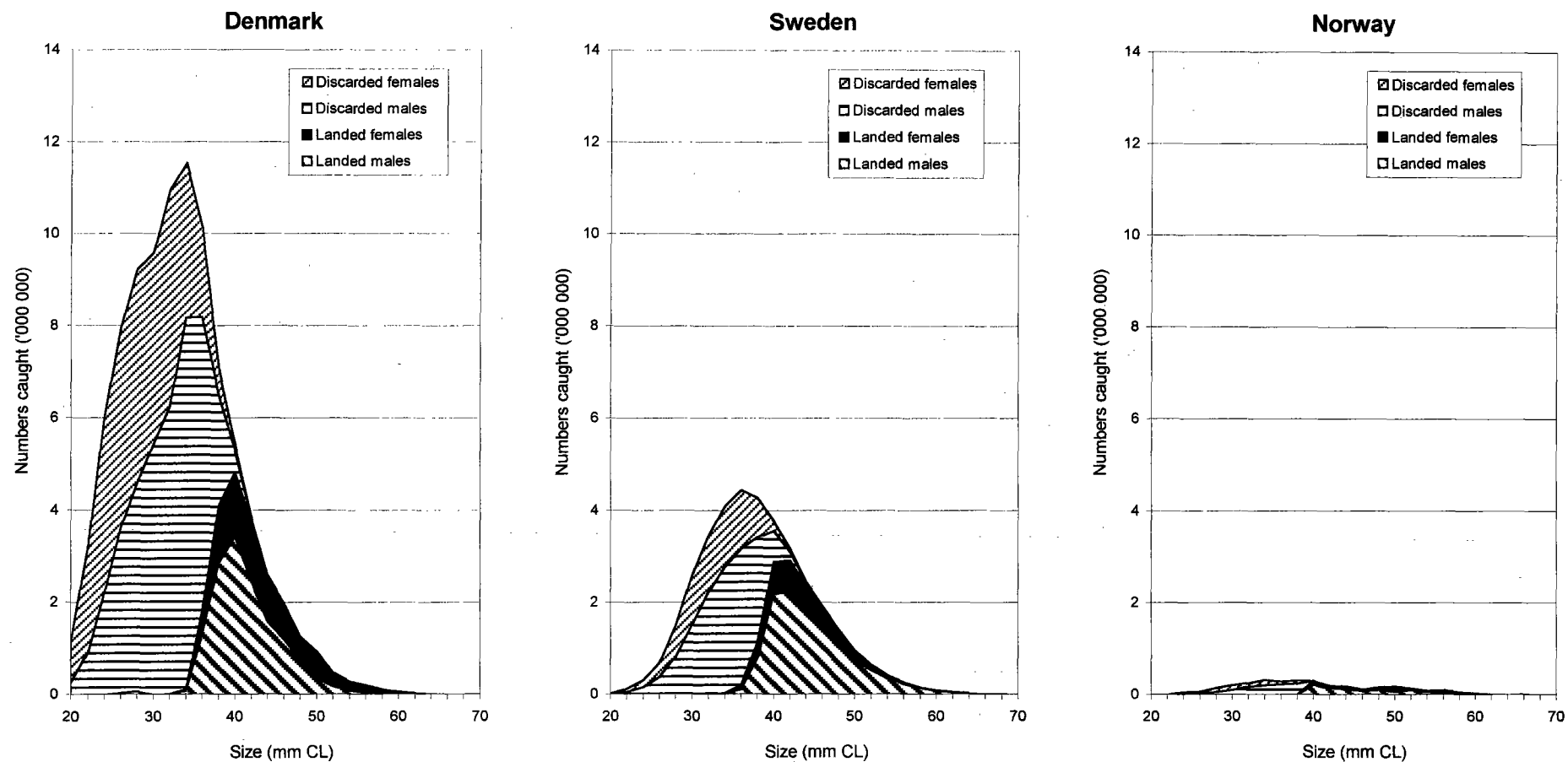
Figure 5.2.7. - Skagerrak (FU 3): Length frequency distributions of Nephrops catches, split by catch fraction (landings and discards) and sex. Data for Denmark, Sweden and Norway shown separately.
