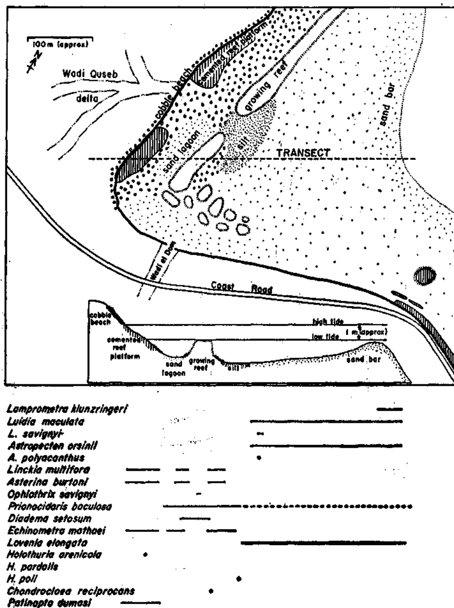
FIG. 3. Sketch of the collecting site at Wadi el Dom in the northwestern Gulf of Suez, with a profile transect of the area and a listing of the echinoderms found. The lines and dots to the right of the echinoderm species show where they occurred with respect to the profile.
