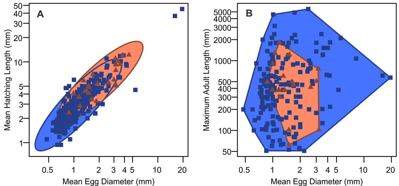
Figure 4. Influence of egg size on later body sizes. A, hatching versus egg size, with 95% confidence ellipses; B, maximum adult size versus egg diameter, with convex hulls. See Supplementary Data for data sources. Red symbols are for spherical eggs with post-fertilization expansion of perivitelline space, whereas blue symbols are for smooth spherical eggs without such expansion or parental care. Note that species with perivitelline expansion have larger hatching size on average but not necessarily the maximum adult size.
