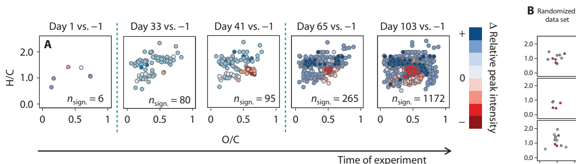
Fig. 3. Molecular differences over time. (A) Exemplary van Krevelen diagrams showing only the molecular formulae (out of 7360) that significantly varied in their intensities over the course of the experiment compared to day –1 for all 10 mesocosm replicates ( P < 0.001 ). The different colors represent differences in normalized relative peak intensity: blue dots indicate an increase in peak intensities, whereas red dots indicate a decrease in peak intensity. Green dashed lines represent time points of phytoplankton blooms. (B) The results are within the statistical error, determined by performing the same test on a randomized data set.
