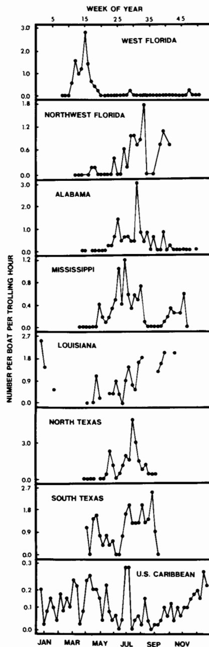
Figure 8.—CPUE by area for king mackerel caught by trolling on Gulf of Mexico and U.S. Caribbean coasts in 1985.
