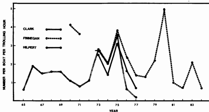
Figure 10.—CPUE by individual charterboat captain in northwest Florida and Alabama, 1965-84.
