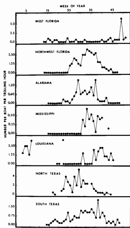
Figure 6.—CPUE by area for king mackerel caught by trolling on the U.S. Gulf coast in 1983.
