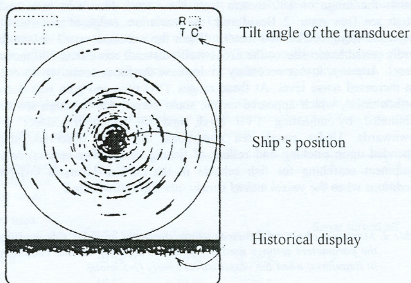
Fig.1. Unwanted echoes caused by surface turbulence on the sonar screen
