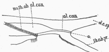
FIG. 13.—Same as fig. 11. Lateral view of posterior part of alimentary canal, etc. \times 280 .
