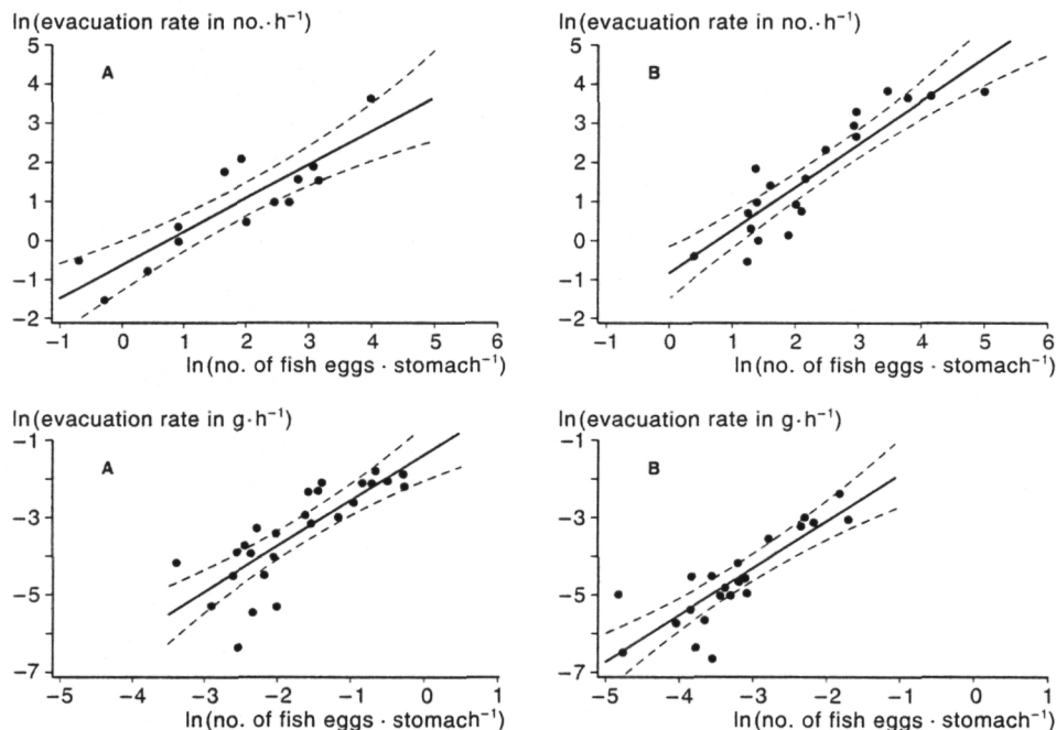
Figure 7 (upper panel). Evacuation rate of fish eggs in numbers (ds/dt). Logarithmic regression of evacuation rate on average number of fish eggs per stomach with 95% confidence limits from combined 24-h surveys and deck-tank experiments. A: herring: slope b = 0.85 , intercept a = -0.64 , r^2 = 0.77 , power function ds/dt = 0.53 \cdot S^{0.85} ; B: sprat: slope b = 1.09 , intercept a = -0.87 , r^2 = 0.80 , power function ds/dt = 0.42 \cdot S^{1.09} .
