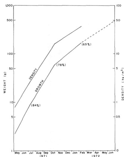
Figure 2.—Growth, rearing density, and survival of hybrid Pacific salmon (♀ O. tshawytscha × ♂ O. gorbuscha ) in a small floating net pen. Pen volume is 2.7\text{m}^3 . Percentage of survivors is in brackets and the broken line indicates growth after transfer to a larger pen.
