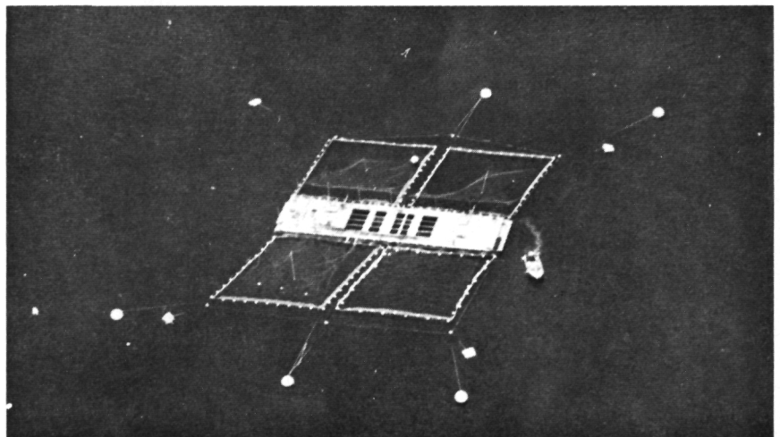
Figure 7. — Aerial view of the pilot salmon farm. Total volume of the four net pens is 7,000m 3 . Market harvest from the 0.1 ha of enclosures was 61.4 mt of Pacific salmon.
