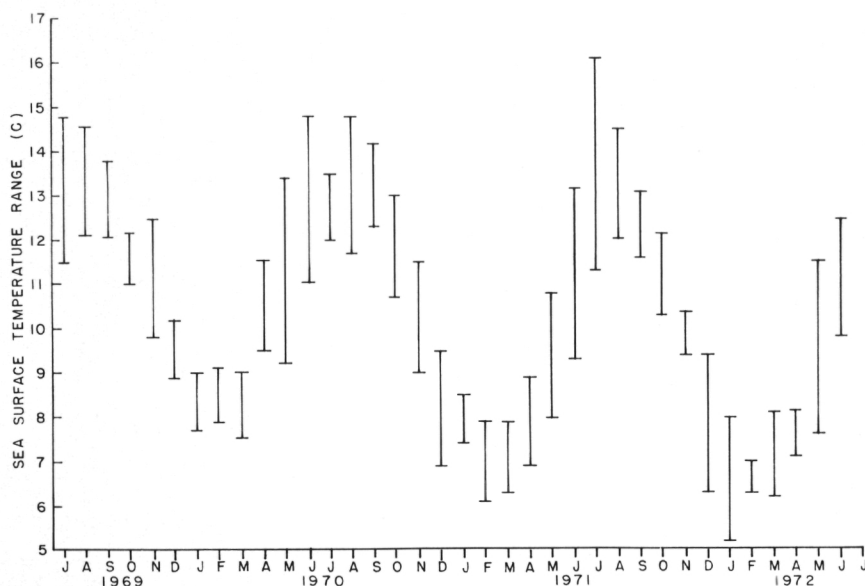
Figure 8.—Records of maximum and minimum monthly sea surface temperatures at Clam Bay, near Manchester, Wash.
