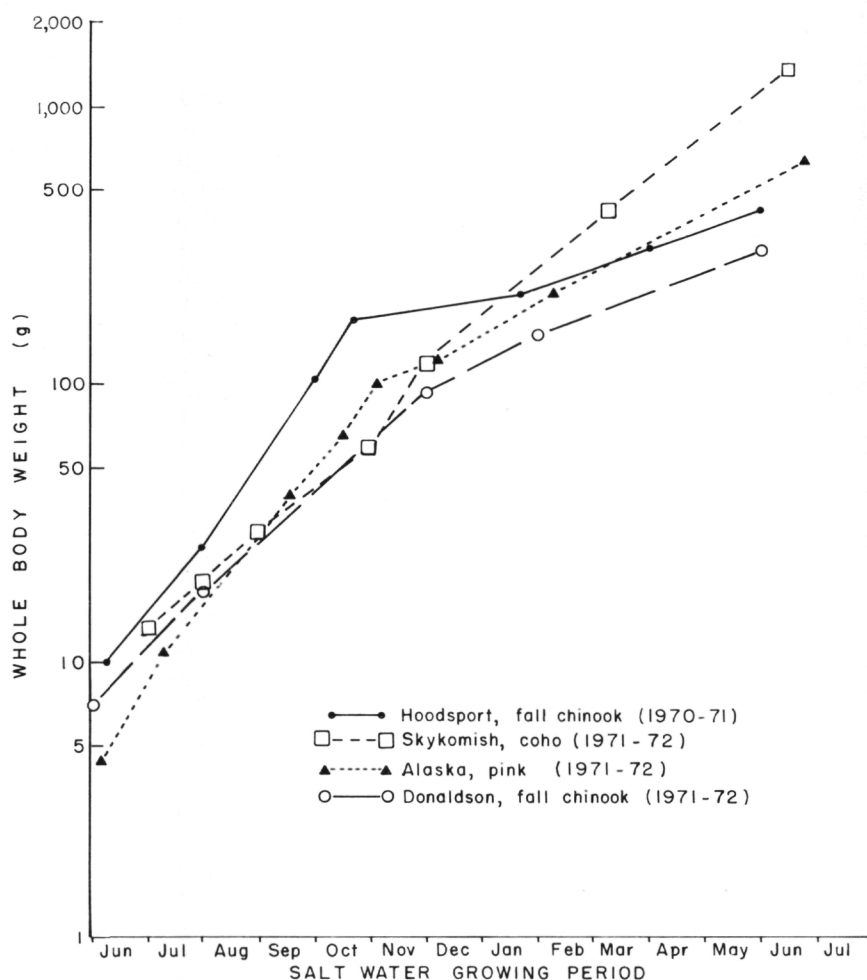
Figure 9.—Growth of three species of Pacific salmon during 1 yr in salt water. Differences between growth of the two stocks of chinook salmon (reared in different years) are believed due to differences between size at entry to salt water, water temperature, and disease influences.
