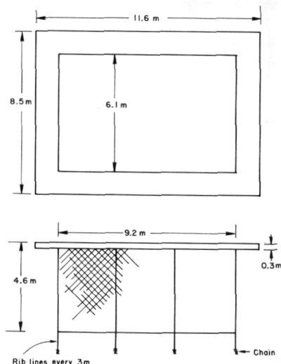
Figure 3.—An experimental production raft and net pen. Raft construction is of lumber, plywood, and Styrofoam billets. Pen volume is 258\text{m}^3 , and production capacity is approximately 4,000 kg of salmon.
