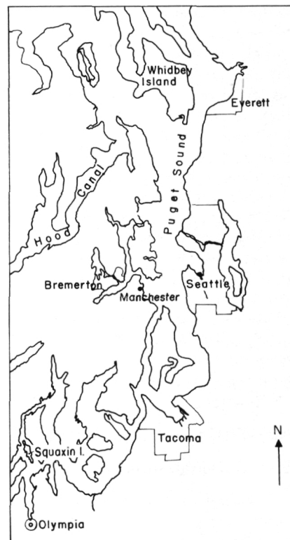
Figure 1.—Puget Sound, Wash. This inland arm of the Pacific Ocean is the site of major activities for the marine culture of Pacific salmon.
