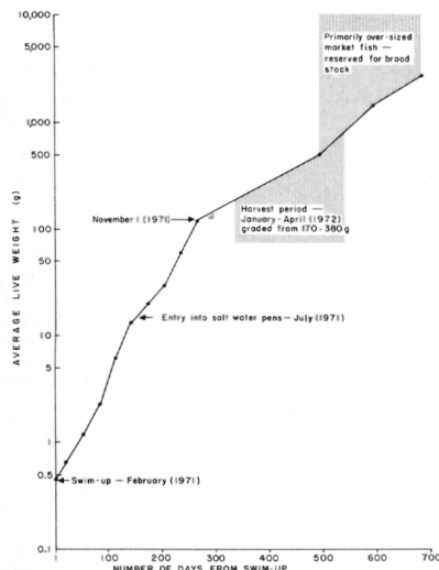
Figure 14. — Accelerated growth of coho salmon from the 1970 brood of Skykomish River hatchery stock.
