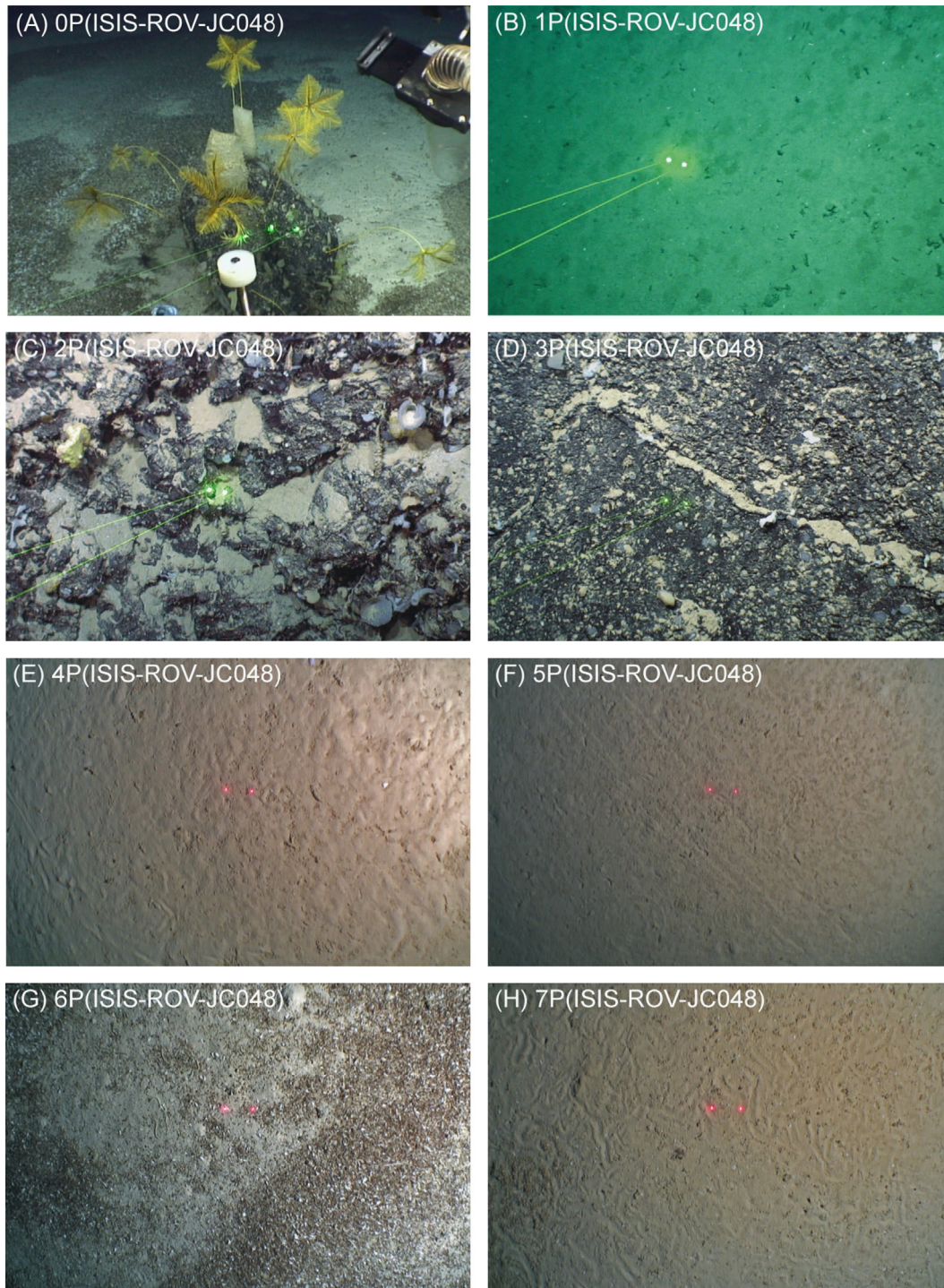
Fig. 10. Images of sea-floor on the MAR taken by ROV Isis cameras during RRS James Cook cruise JC048: (A) rock outcrop surrounded by sediment on a nominal 10° slope at the SE ECOMAR superstation (note contrasting areas of pale fine sediment and areas of coarse superficial deposit of pteropod shells; forward-facing camera looking obliquely downwards), (B) soft sediment talus covering 30° slope at the NE superstation (forward-facing camera looking obliquely downwards), (C) rock outcrops with sponges attached on a steep slope at the NE superstation (note sediment cover on horizontal ledges; camera looking horizontally at a steep cliff face), (D) rock surface at the NE superstation (camera looking horizontally at a vertical cliff face), (E) soft sediment covering an 8–12° slope at the NE superstation, (F) soft sediment covering a flat area at the NE superstation, (G) soft sediment covering an 8–12° slope at the SE superstation (note the contrast between fine sediment and coarser shell deposits), (H) soft sediment covering a flat area at the SE superstation. The camera is looking vertically downwards below the ROV except where indicated. Paired parallel laser beams 10 cm apart provide a reference scale. Note extensive bioturbation or lebenspuren.
