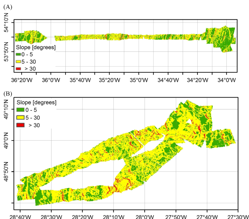
Fig. 5. Swath bathymetry transects across the MAR between the ECOMAR superstations surveyed during RRS James Cook (cruise JC011) showing slopes in three categories: 0–5°, 5–30° and > 30° for (A) the Northern transect between the NW and NE superstations, (B) the Southern transect between the SW and SE superstations.
