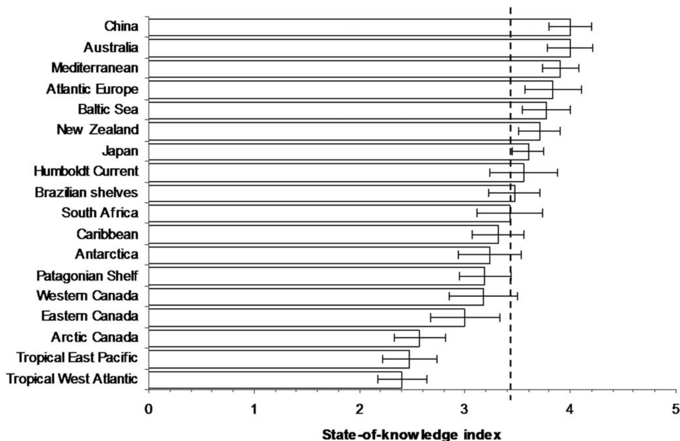
Figure 3. The regions ranked by their state-of-knowledge index (mean \pm standard error) across taxa. Dashed line represents the overall mean.
