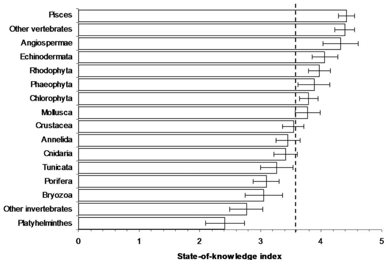
Figure 4. The taxonomic groups ranked by their state-of-knowledge index (mean \pm standard error) across regions. Dashed line represents the overall mean. doi:10.1371/journal.pone.0012110.g004
