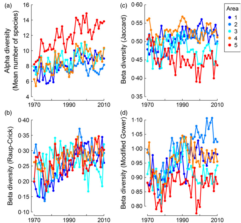
Fig. 3. Annual values from 1970 to 2010 within each of five sub-areas across the Scotian Shelf (see legend) for each of four biodiversity variables calculated from all fishes caught in trawl sets, excluding cod: (a) alpha diversity (mean number of species); mean distance-to-centroid (beta diversity) based on (b) Raup–Crick; (c) Jaccard; or (d) modified Gower dissimilarity measures.
