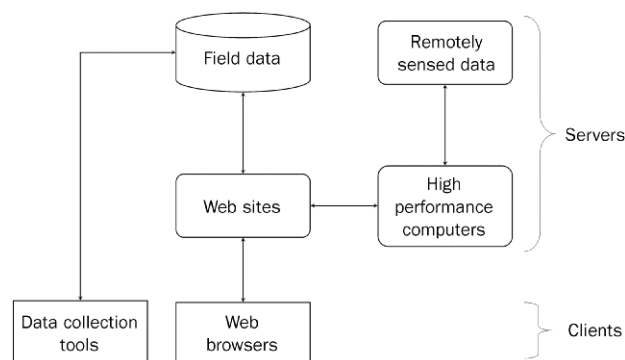
Figure 1. Architecture for an invasive species cyberinfrastructure.
