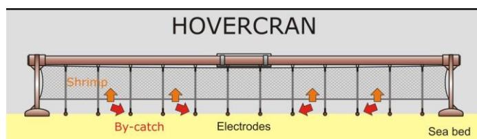
Figure 3 Principle of the Hovercran trawl where electrodes stimulate the shrimp to jump over a raised footrope into the gear
