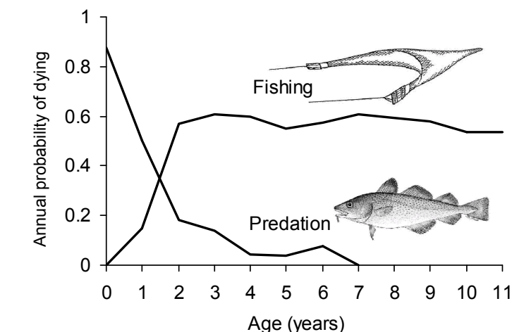
Figure 10. Annual probability of dying from predation or fishing for the different age groups of North Sea cod ( Gadus morhua ), average 1987–1994 (from Kolding and van Zwieten, in press)
