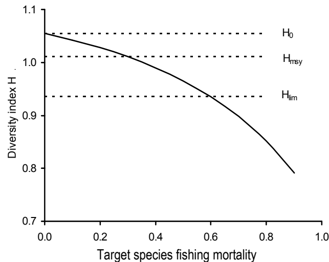
Figure 7. General relationship between diversity and fishing intensity when fishing is selective. H_0 , H_{msy} , and H_{lim} are diversity reference points corresponding to target species biomass at B_0 , B_{msy} , and B_{lim} when no fishing mortality occurs in other species (Zhou et al. , unpublished data)
