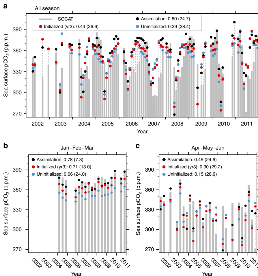
Figure 4 | Observed and model simulated monthly mean ocean surface p\text{CO}_2 in western SPG region. (a) All season time series, (b) only January–February–March are shown and (c) only April–May–June are shown. The SOCAT observations 36 are shown with grey bars, and model output of assimilation, uninitialized simulations and initialized simulations at a lead time of 3 years (yr3) are shown in black, blue and red dots, respectively. The grey dashed lines connect outlier dots with the grey bars to make the comparison clearer. The numbers in legend are correlation coefficients and root mean squared error (in brackets) between model simulations and SOCAT observations. For the all season time series in a the correlations of the assimilation and initialized simulations at lead time of 3 years are significantly larger than that of the uninitialized simulations at 95% significant level based on a bootstrap test. Note the SOCAT observational data are not continuously distributed in space and time; the model simulations are averaged over the grid points where SOCAT data are available.
