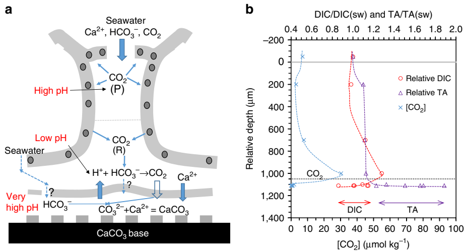
Figure 3 | Conceptual model of coral calcification and \text{CO}_2 transport mechanism and distributions of internal [\text{CO}_2] and relative DIC and TA to seawater values. (a) Illustrative model and (b) concentration distributions. Dark circles are photosynthetic endosymbionts. P stands for photosynthesis, R for respiration, and sw for seawater. In (b), for DIC (red line) and TA (purple line) the calculated ranges of possible concentrations inside the calcifying fluid are provided based on calculations of all species from Supplementary Table 1.
