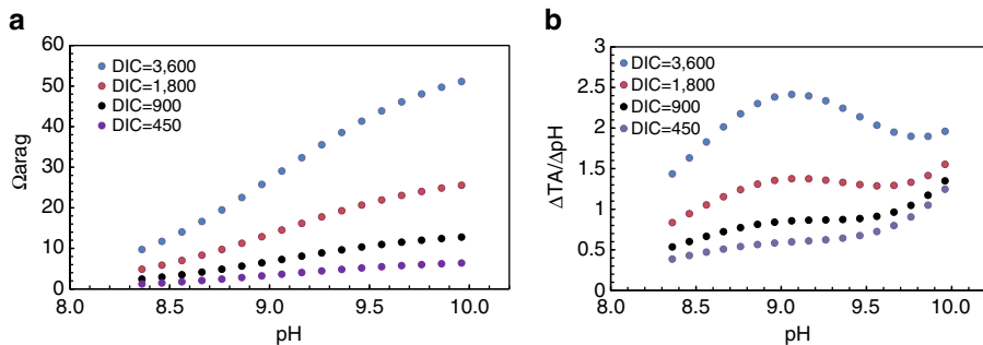
Figure 4 | Aragonite mineral saturation state ( \Omega_{\text{arag}} ) and buffer index in the coral calcifying fluid as functions of pH and [DIC]. (a) \Omega_{\text{arag}} and (b) buffer index. The buffer index is given as mmol kg -1 of \text{H}^+ pumping ( \text{H}^+ loss or TA gain) per unit of pH upregulation. This index is calculated numerically with CO2SYS (ref. 37) (see Methods section). Here [DIC] = 1800 μmol kg -1 is roughly the same as seawater value. pH is on the NBS scale.
