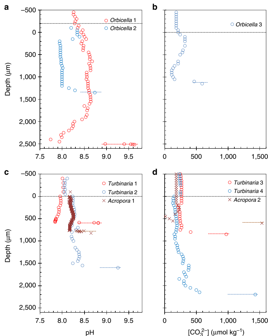
Figure 2 | Coral internal pH and [\text{CO}_3^{2-}] profiles through the polyp mouths. (a) pH and (b) [\text{CO}_3^{2-}] of Orbicella faveolata corals. (c) pH and (d) [\text{CO}_3^{2-}] of Turbinaria reniformis and Acropora millepora corals. Dashed black lines indicate the top of the polyp mouths. Colored dashed lines roughly indicate the location of the calcifying fluid and differ in depth for each polyp.
