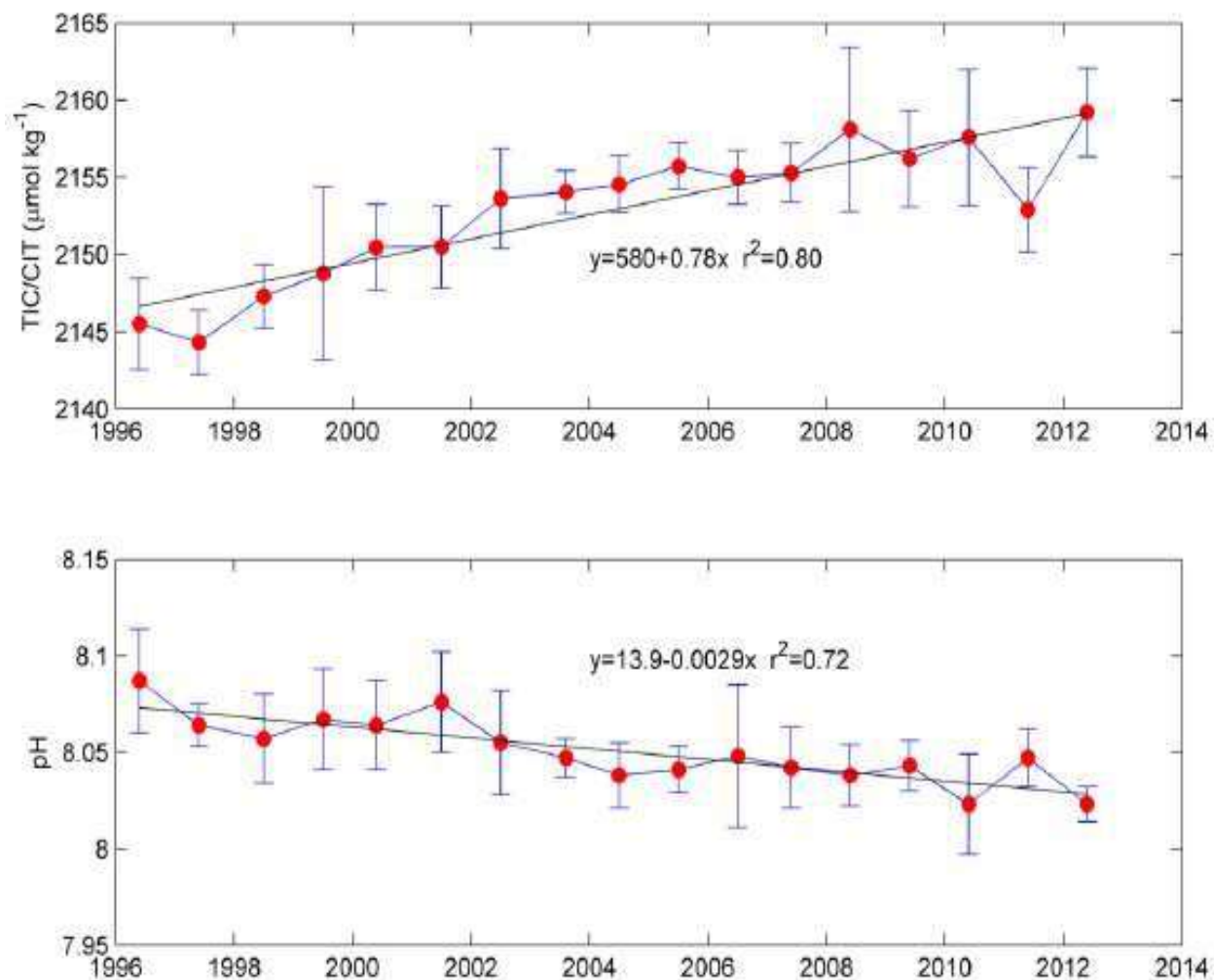
Figure 6. Time series of total inorganic carbon (TIC) and pH (top panel refers to TIC, bottom panel to pH) in the 150–500 m depth range and corresponding regression lines for stations in the central part of the Labrador Basin for the period 1996–2012. In 2012, pH is a direct measurement because alkalinity measurements were not available due to an instrument failure (Yashayaev et al. 2013)
